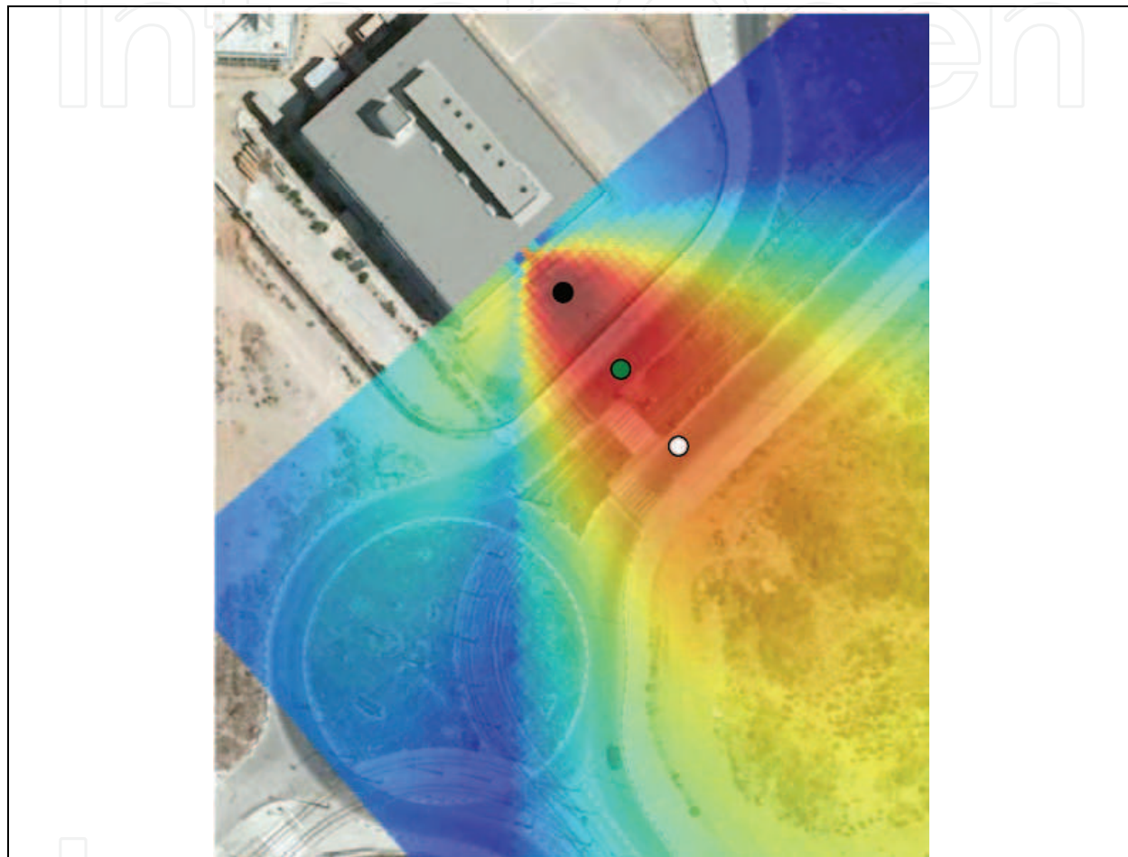
Fig. 9. Power distribution within the communication zone in the test area.
