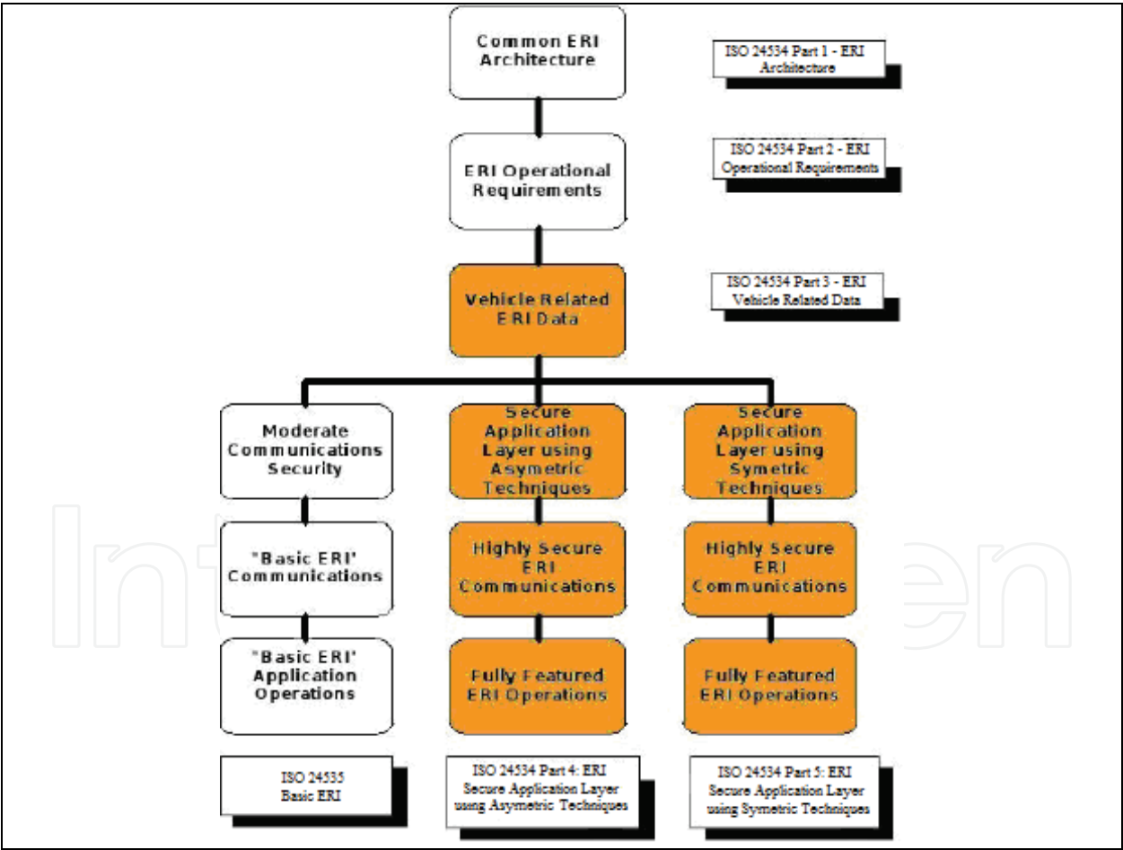
Fig. 4. Functional pile of the ERI system (includes different standards) The protocol was implemented for each application scenario, originally planned as a set of messages to be used in each application and sequence. In order to apply the protocol, the ERI standards suggest DSRC technology, but several wireless technologies more and their
