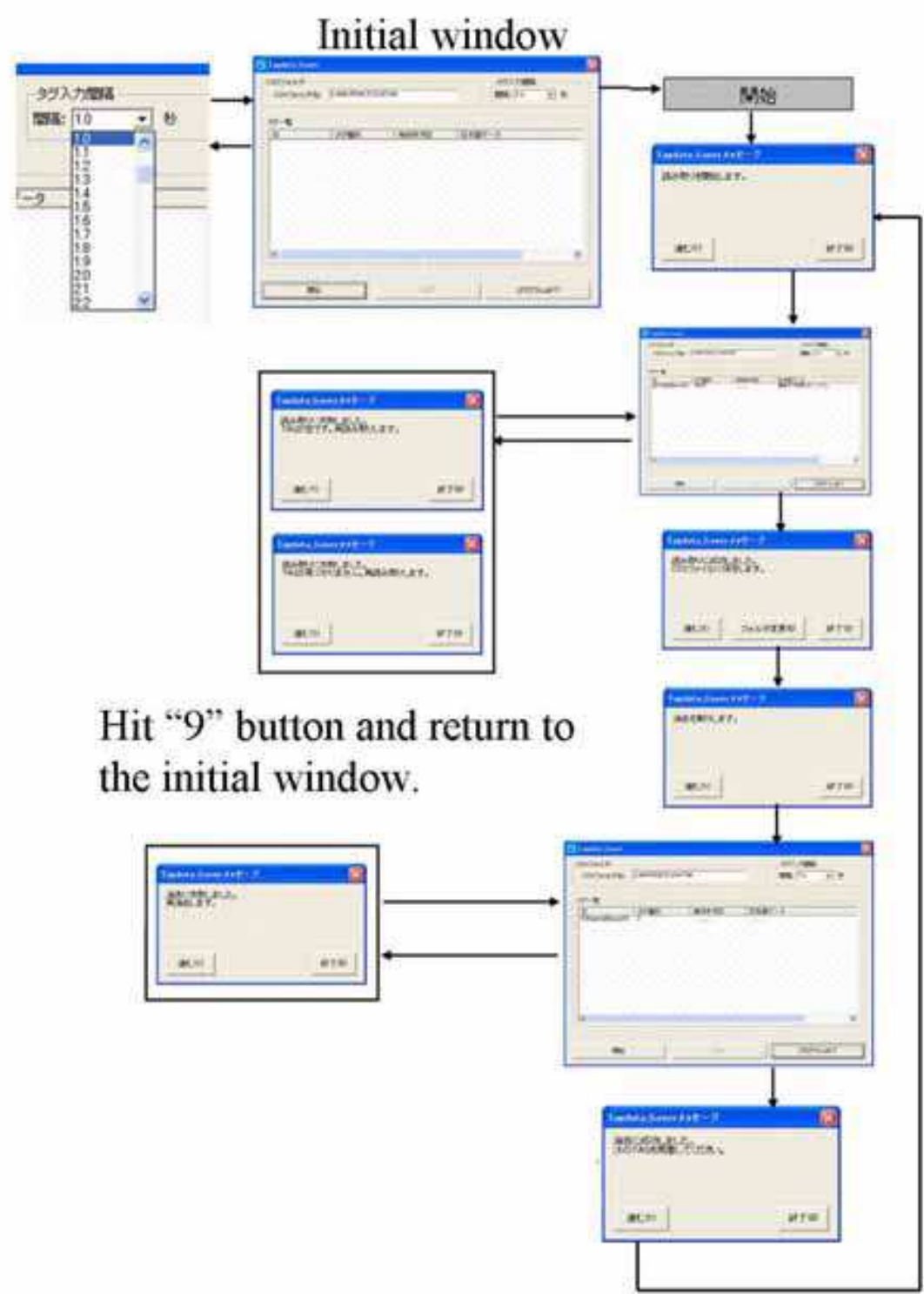
Fig. 9. Screen State Transition Diagram of the Retrieval Function
