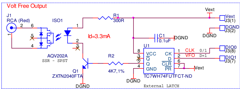
Fig. 23. Volt Free Output The Volt Free Output extension is only recommended for applications where an external power supply is used.
