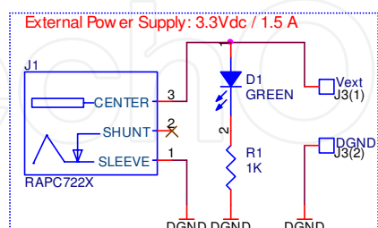
Fig. 17. The Tag4M External Power Supply
