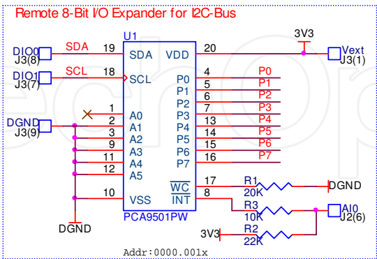
Fig. 29. Remote 8-Bit IO Expander for I 2 C Bus
