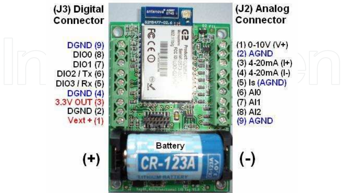
Fig. 3. Tag4M I/O Connector Blocks
