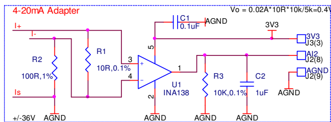
Fig. 25. 4-20 mA Current Input Circuit
