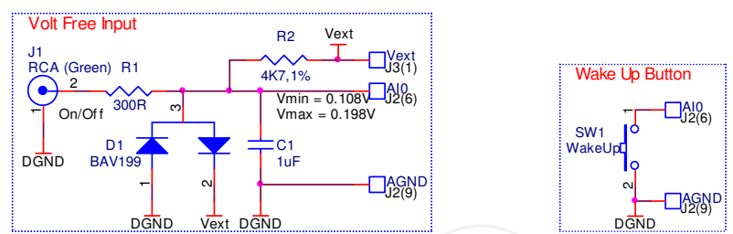
Fig. 22. Volt Free Input and Wake Up Button The wake up button implementation is a cheaper version of the volt free input board, which does not offer protection against signal spikes. The Volt Free Output extension presented in Figure 23 is used to control a light source, AC/DC motor, etc. The extension board circuitry is based on a solid state relay AQRV202A that works in both AC and DC at 60V, 0.4A, and has optical isolation (Panasonic, 2005). The external latch, TC7WH74 IC, is necessary to keep the output unchanged while the tag is in sleep mode which sets signal lines CLK and VFO to floating state (Toshiba, 2001).
