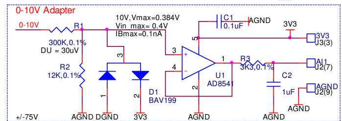
Fig. 24. 0-10V Voltage Input Circuit The voltage conversion formula from 0-10V in 0-0.4V is (1):
