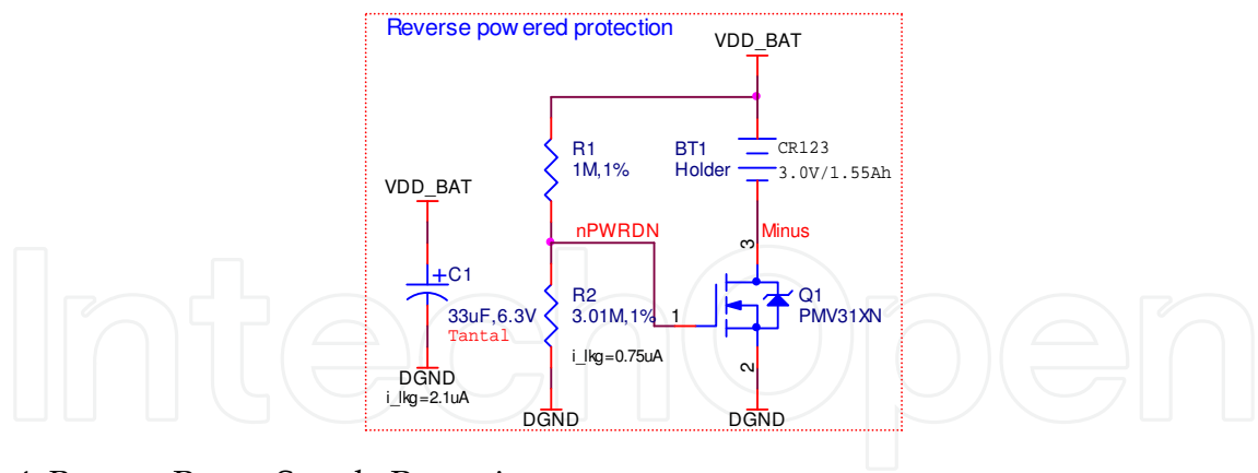
Fig. 4. Reverse Power Supply Protection
