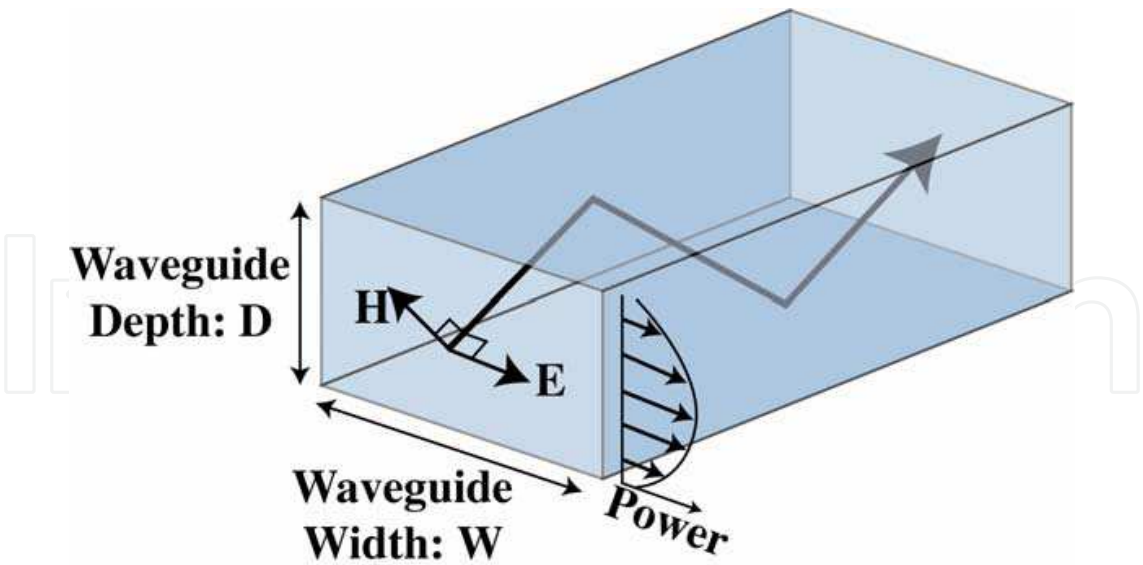
Fig. 7. Assumed model for analysis of propagation characteristics of hollow waveguide.
