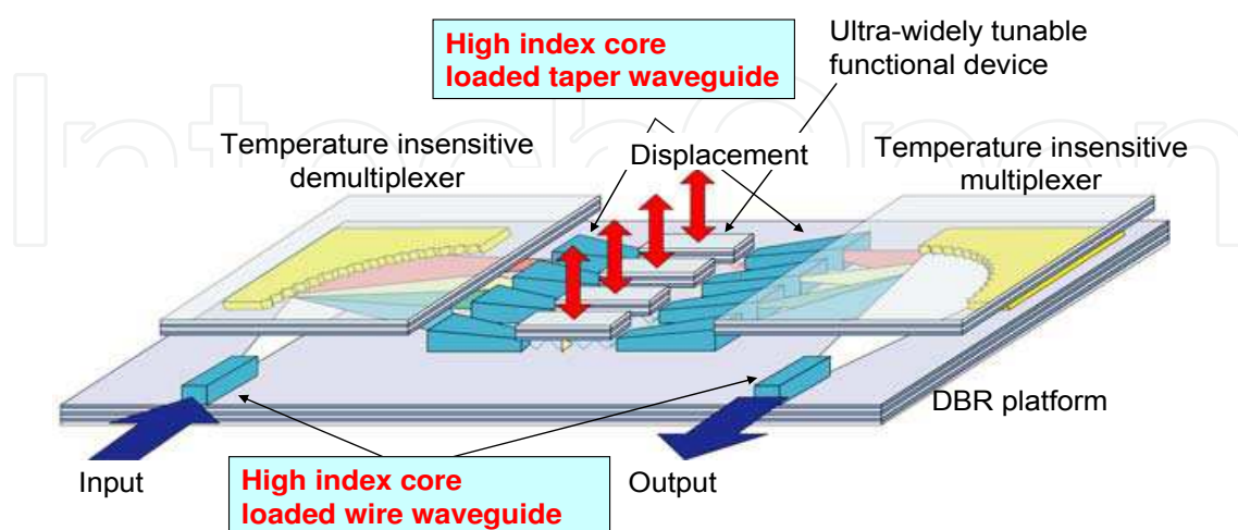
Fig. 16. Image of the scheme of reconfigurable photonic integrated circuit with tunable hollow waveguide using a high index core loaded waveguides for WDM applications.
