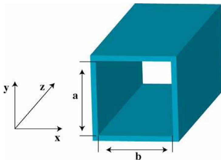
Fig. 4. Assumed 3D hollow waveguide model for analysis.
