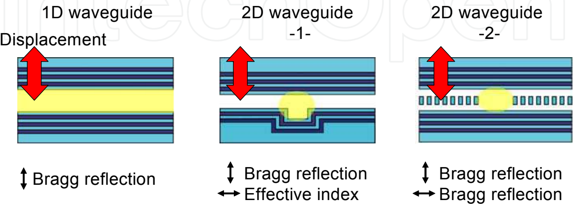
Fig. 3. Tunable Hollow optical waveguide structures [38]-[40].
