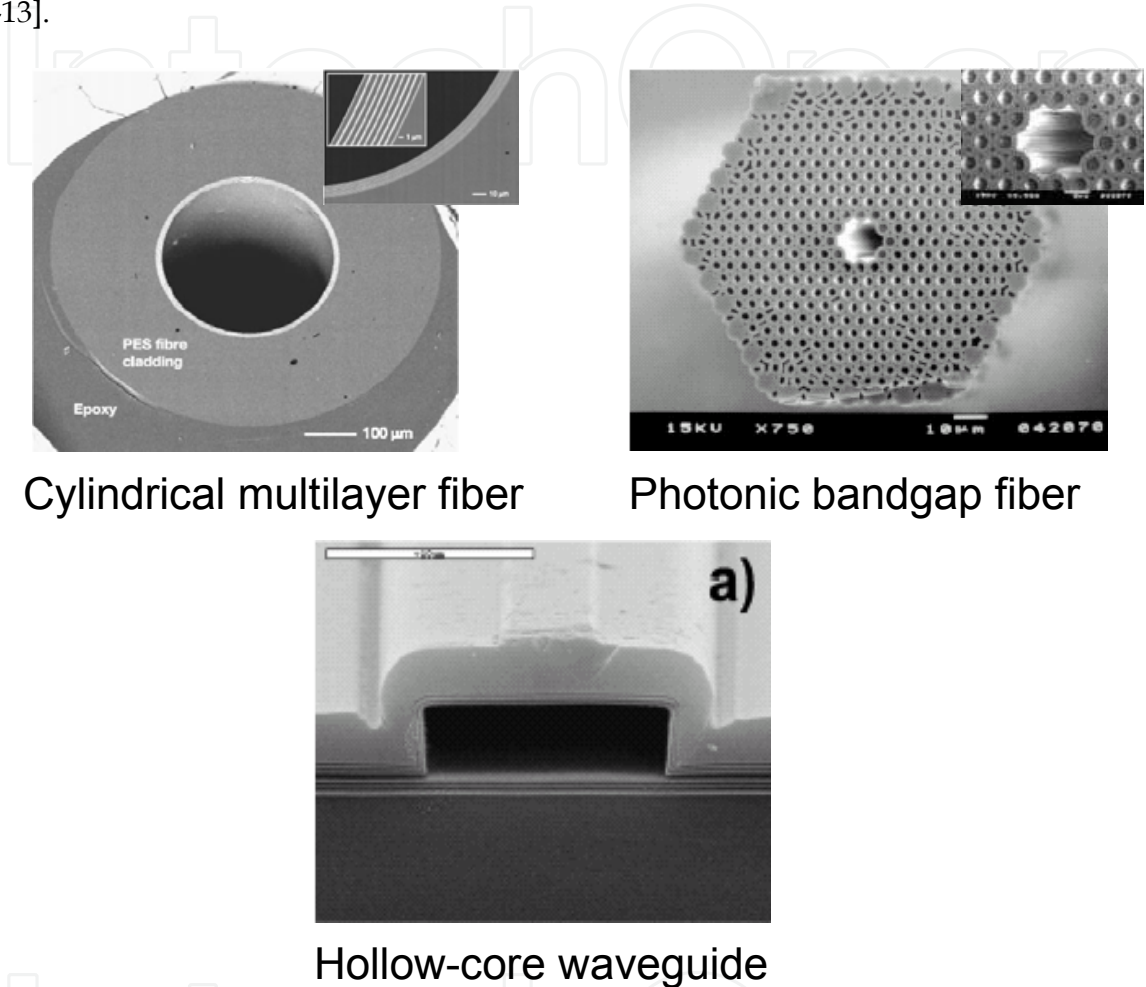
Fig. 1. Various air-core guiding structures [1-3].
