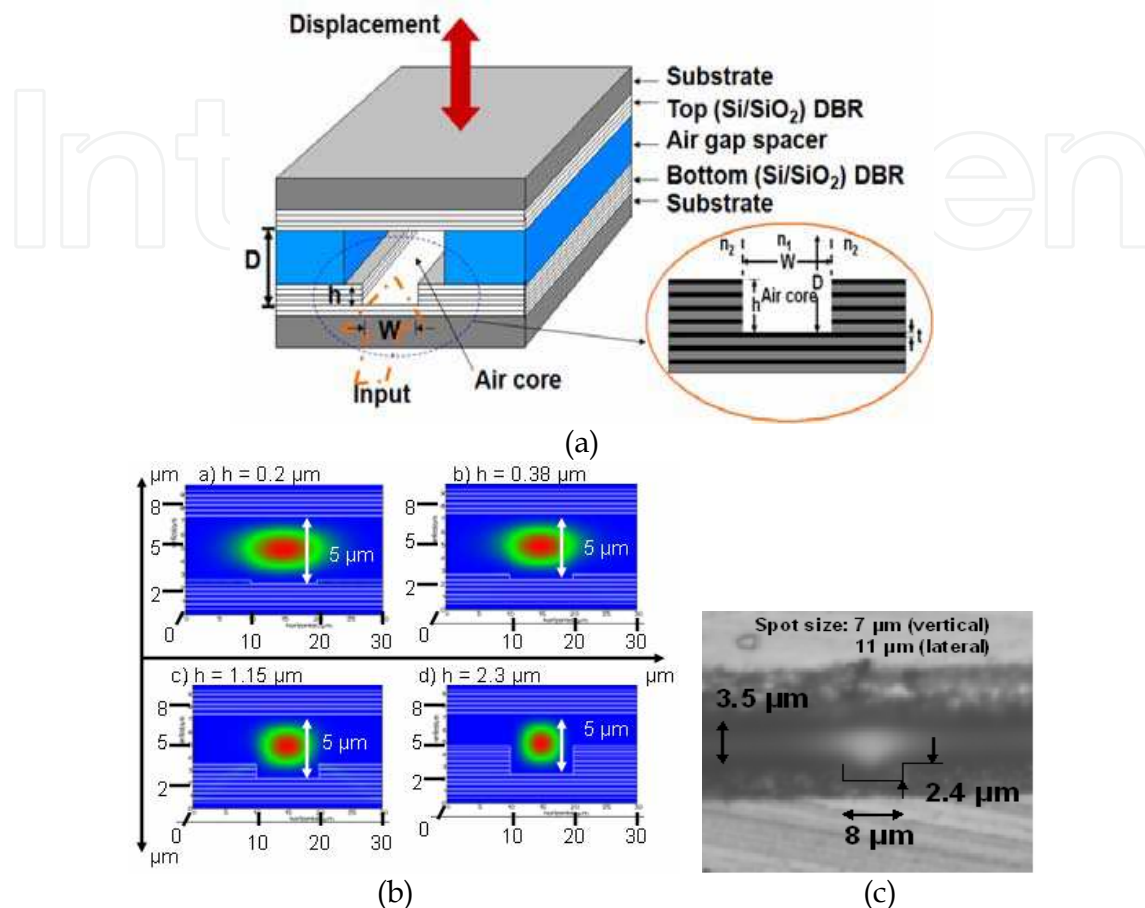
Fig. 9. (a) Schematic of tunable 3D hollow waveguide. All the layers in top and bottom DBR mirrors are quarter wavelength thick except the first silicon layer in bottom DBR just under the air core which we call phase matching layer with thickness t , shown in inset. (b) Computed effect of step-height on mode-field distributions at an air core thickness D = 5 \mu\text{m} and step width W = 10 \mu\text{m} , and (c) measured near field pattern for TE-mode.
