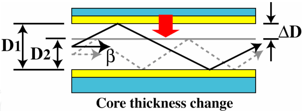
Fig. 6. Conceptual diagram of propagation constant tuning.
