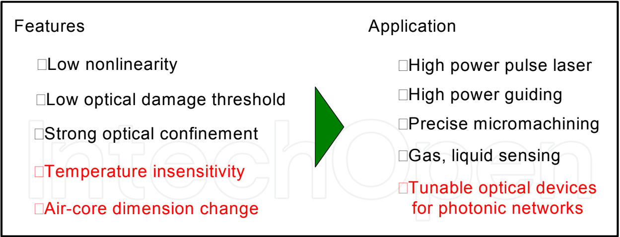
Fig. 2. Application of air-guiding waveguides [11-13].
