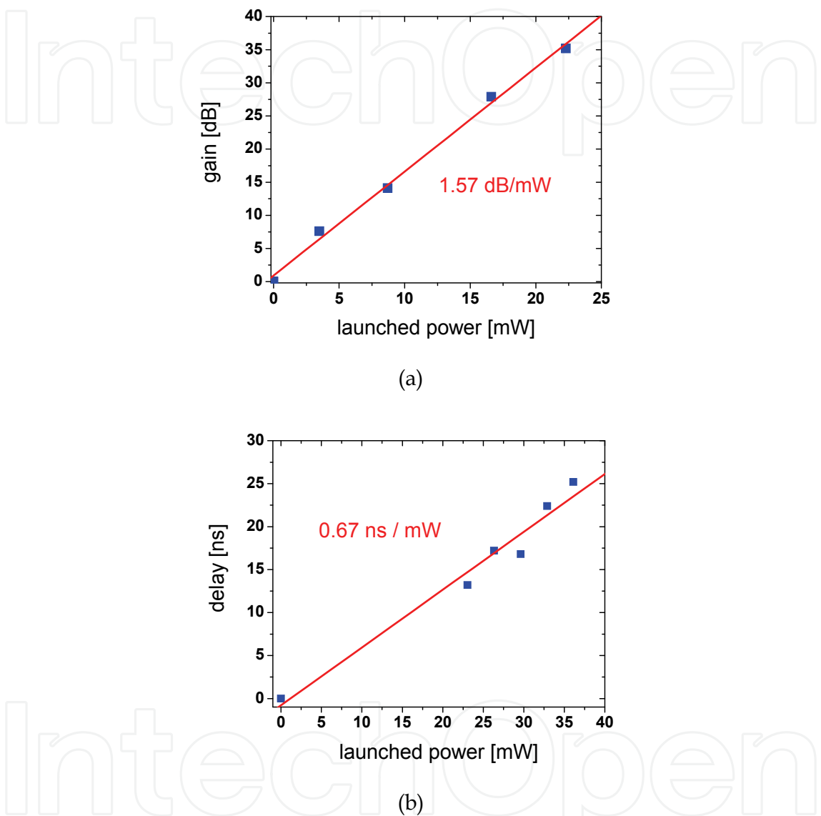
Fig. 18. (a) Gain and (b) pulse delay measurements in 10-m long As 2 S 3 fiber at 1548 nm.
