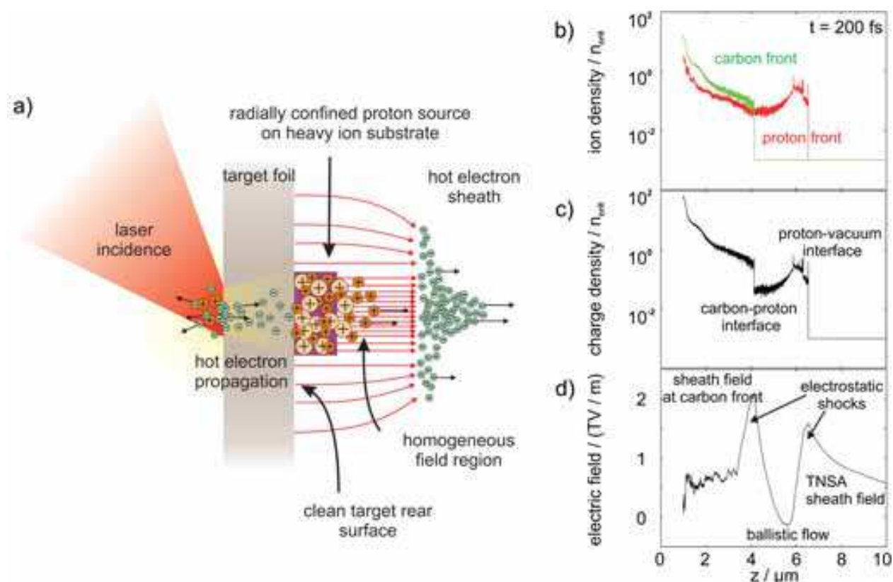
Fig. 14. The schematics of the Confined TNSA process (a) and results from a simulation of the acceleration process (b)–(d) at 200 fs. Simulation data courtesy of A.P.L. Robinson (Pfotenhauer, 2009; Robinson et al., 2009).
