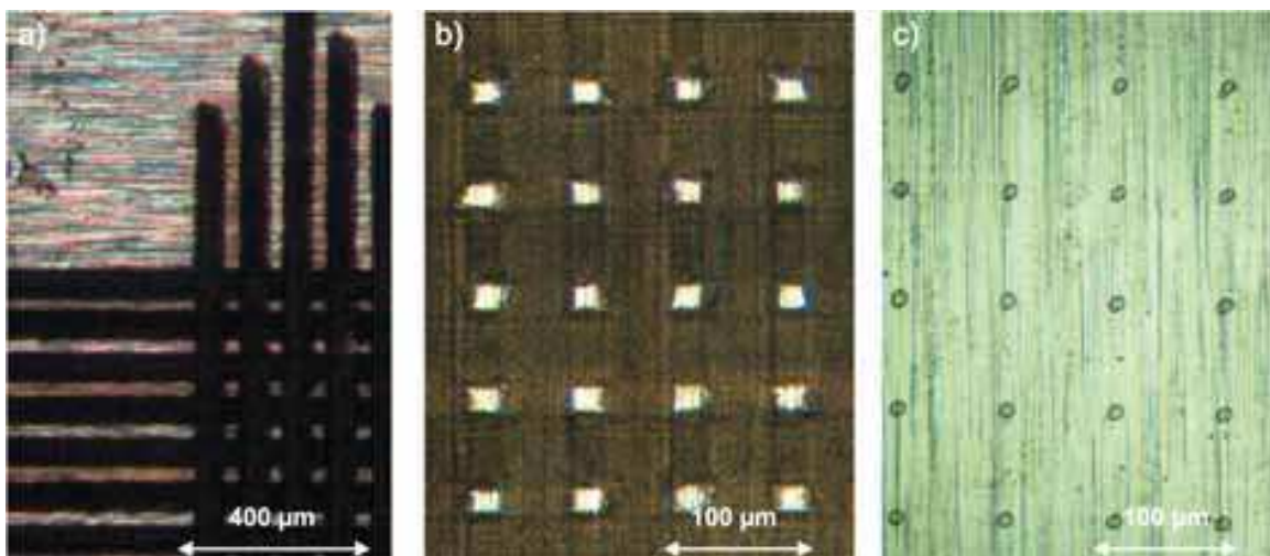
Fig. 16. (a) + (b) Fabrication of microstructured targets via fs-laser ablation. For the fabrication of microstructured targets suitable for Confined TNSA, a layer of polymer (PMMA) with 50 – 1000 nm thickness was first deposited to titanium foils via spin coating. From the polymer-covered surface, small square dots of 20 \times 20 \mu\text{m}^2 extent and 80 \mu\text{m} separation were “carved out” with the help of a femtosecond laser system. Fig. (a) clearly shows the perpendicular carving traces ranging into the polymer. Note the well-defined carving edges typical for fs-ablation. (c) Lithography targets. Round dots of 10 \mu\text{m} diameter with 80 \mu\text{m} separation were generated via UV-lithography with a pulsed excimer laser. This alternative technique allows for a more flexible fabrication of micro-dots, which are, however, considerably more sensitive to target cleaning than those produced with the femtosecond system.
