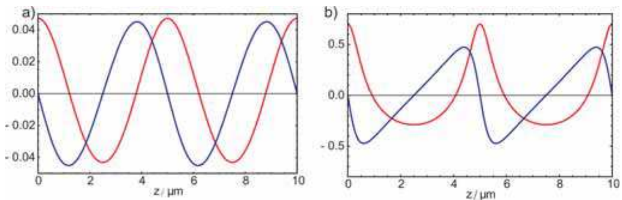
Fig. 3. Electron density perturbation \delta n_e/n_e (red) and longitudinal electric field E_{\text{wake}}/E_p (blue) for (a) a weakly relativistic laser pulse ( a_0 \sim 0.3 ) and (b) a relativistically intense pulse ( a_0 \sim 1 ) in a plasma with 5 \mu\text{m} plasma wavelength. Calculated according to Sec. 4.1 in (Gibbon, 2005).
