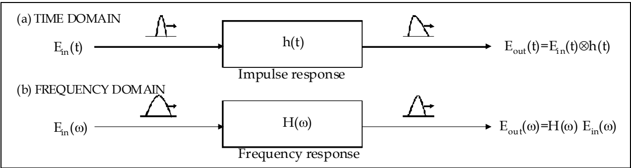
Fig. 1. Pulse shaping by linear filtering. (a) Time domain view. (b) Frequency domain view In the frequency domain, the filter is characterized by its frequency response H(\omega) . The output of the linear filter E_{out}(\omega) is the product of the input signal E_{in}(\omega) and the frequency response H(\omega) -i.e.,
