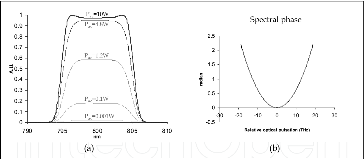
Fig. 7. Simulation of acousto-optic diffraction for (a) spectral amplitude, (b) spectral phase. The first order can then be used to precompensate the saturation within few percents but exact pulse shaping requires to monitor and loop on the spectral amplitude. The spectral phase is automatically conserved through the Bragg phase matching condition.
