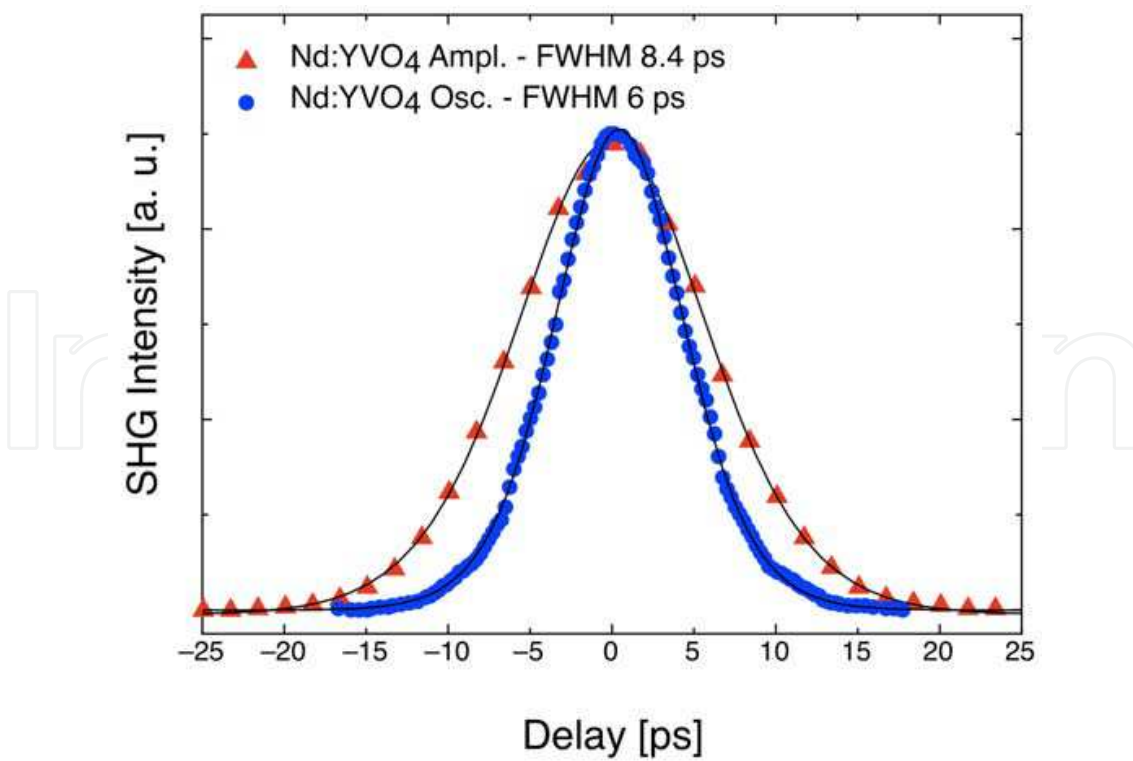
Fig. 17. Autocorrelation traces of both master oscillator (circles) and amplified pulses (triangles). Also shown the sech 2 experimental data fitting.
