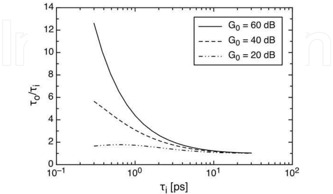
Fig. 2. Output pulse width broadening as a function of the seed pulse duration. Three small-signal gain levels are considered. Injected seed energy of 1 nJ is typical of most picosecond seeders.
