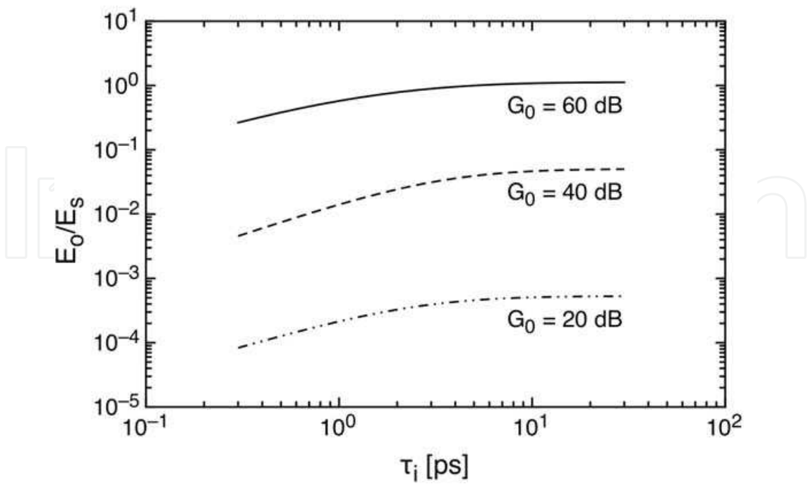
Fig. 3. Output energy as a function of the seed pulse width, for three small-signal gain levels. Injected seed energy is 1 nJ.
