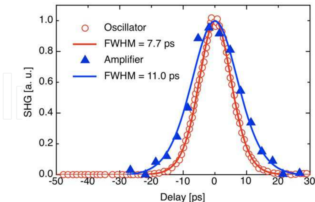
Fig. 12. Pulse autocorrelation of the oscillator (circles) and amplified (triangles) beam. Also shown are the best-fit traces corresponding to \text{sech}^2 intensity envelope.
