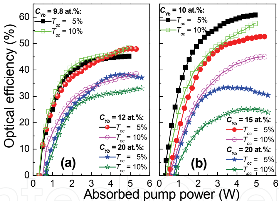
Fig. 5. Optical efficiencies of (a) Yb:YAG ceramic and (b) Yb:YAG single crystal miniature laser as a function of absorbed pump power for different Yb concentrations and transmissions of the output coupler.
