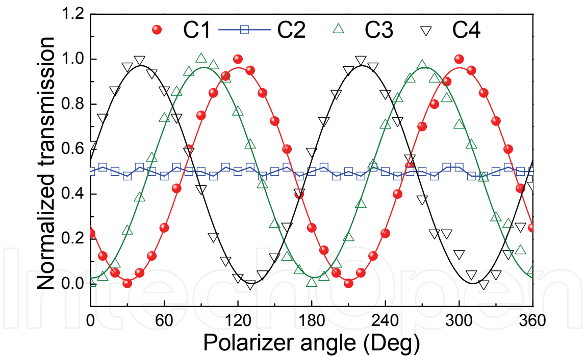
Fig. 10. Polarization states of passively Q-switched Yb:YAG/Cr,Ca:YAG microchip lasers. The solid lines show the sine function fitting of the experimental data.
