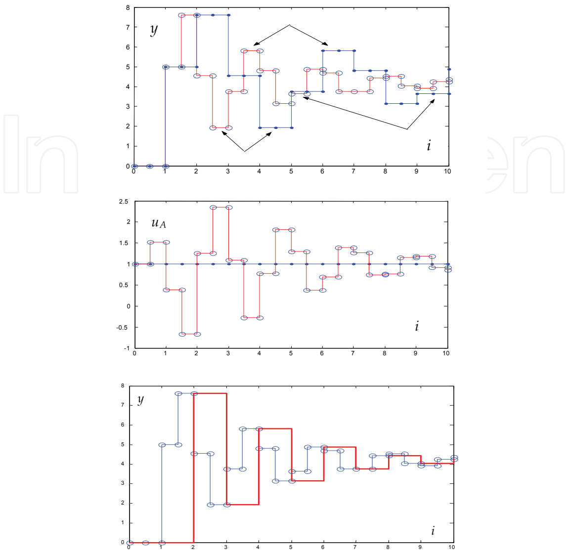
Fig. 5. Upper figure: the reference response of system (6) to signal u(i)=1(i) - curve distinguished by “.” - and the speeded response of system (6) obtained as output signal of structure in Fig. 4 - curve distinguished by “o”. Note, that consecutive amplitudes of both responses are identical (compare chosen referring amplitudes indicated by arrows). Below: reference input u(i)=1(i) and input signal u_A(i) of system (6) when included to structure in Fig. 4 (or in Fig. 2) as SYSTEM. The lowest position: the speeded response of system (6) obtained as output of structure in Fig. 4 - curve distinguished by “o” - and simplified result of scaling with sample time T - heavy line. Note, that every second amplitude of perfectly scaled output y(iT') is equal to respective amplitude of simplified result of scaling for sample time T .
