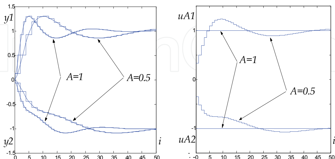
Fig 8. Result of scaling of outputs y_1(t) , y_2(t) (solid lines – responses of system to excitations u_{A1}, u_{A2} , staircase lines- responses of discrete-time model of system) and discrete-time signals u_{A1} , u_{A2} supplying system.
