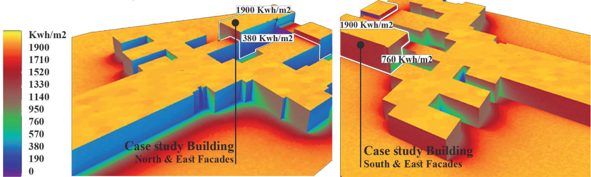
Figure 2. Solar radiation analysis on building envelope.
