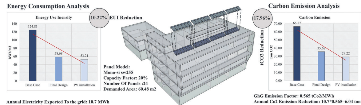
Figure 10. Energy savings and CO 2 emissions reduction by PV installation.
