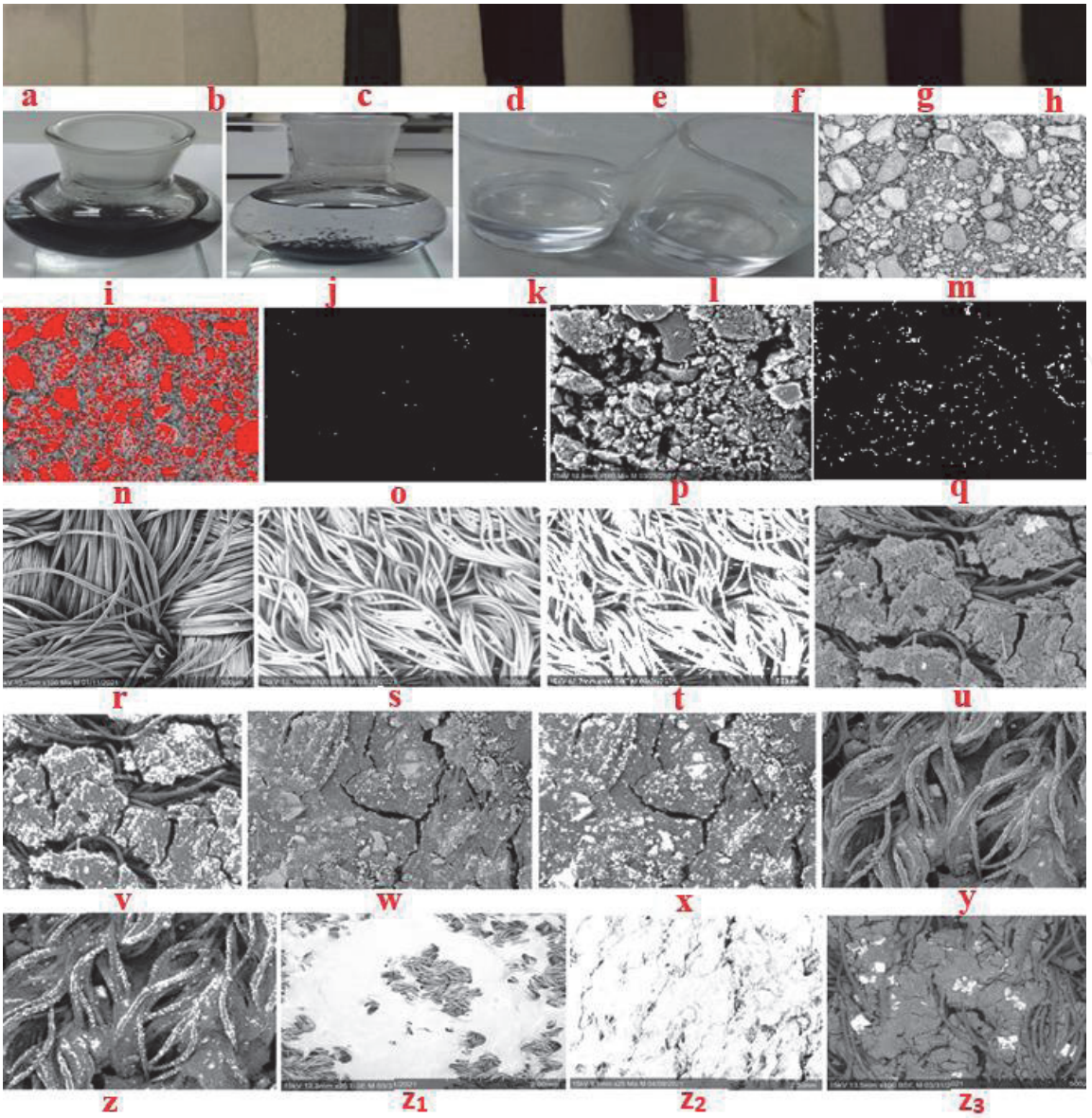
Figure 6. Photograph of treated and untreated fabric (a-h), CBP and TPU-DMF derivative solution (i-l), SEM and color thresholding image of treated and untreated PA 6,6 fabric (m-z 3 ).
