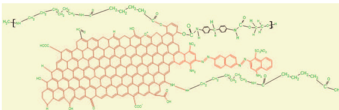
Figure 10. Coupling of CBP-TVRR-TPU-DMF treated PA-6,6.
