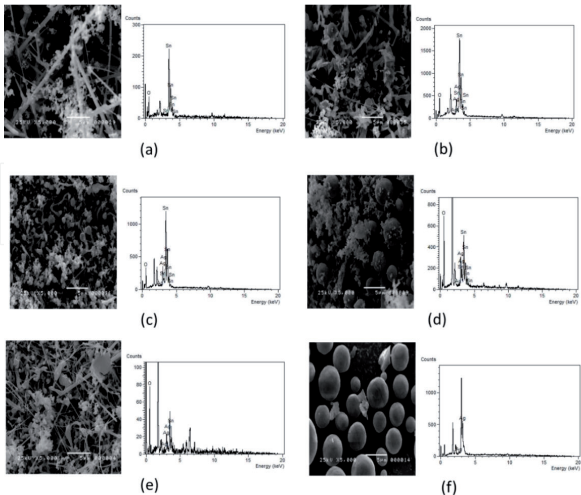
Figure 4. Representative sample of \text{Ag/SnO}_2 with different ratio. ( \text{Ag:SnO}_2 ) (a) 0:5, (b) 1:4, (c) 2:3, (d) 3:2, (e) 4:1, (f) 5:0. Pictures were retrieved from [23].
