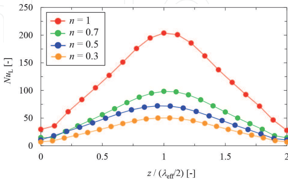
Figure 8. Axial variation in the local Nusselt number ( Nu_L ) along the surface of the outer cylinder at Re_{eff} = 158 [23]. \lambda_{eff} is the wavelength of Taylor cells.
