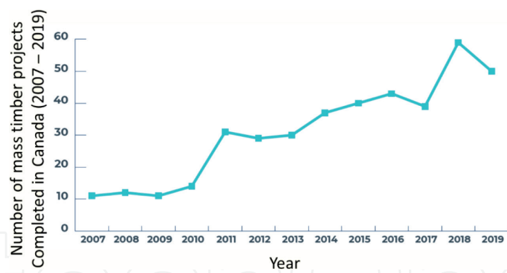
Figure 20. The number of completed mass timber projects per year in Canada [30].
