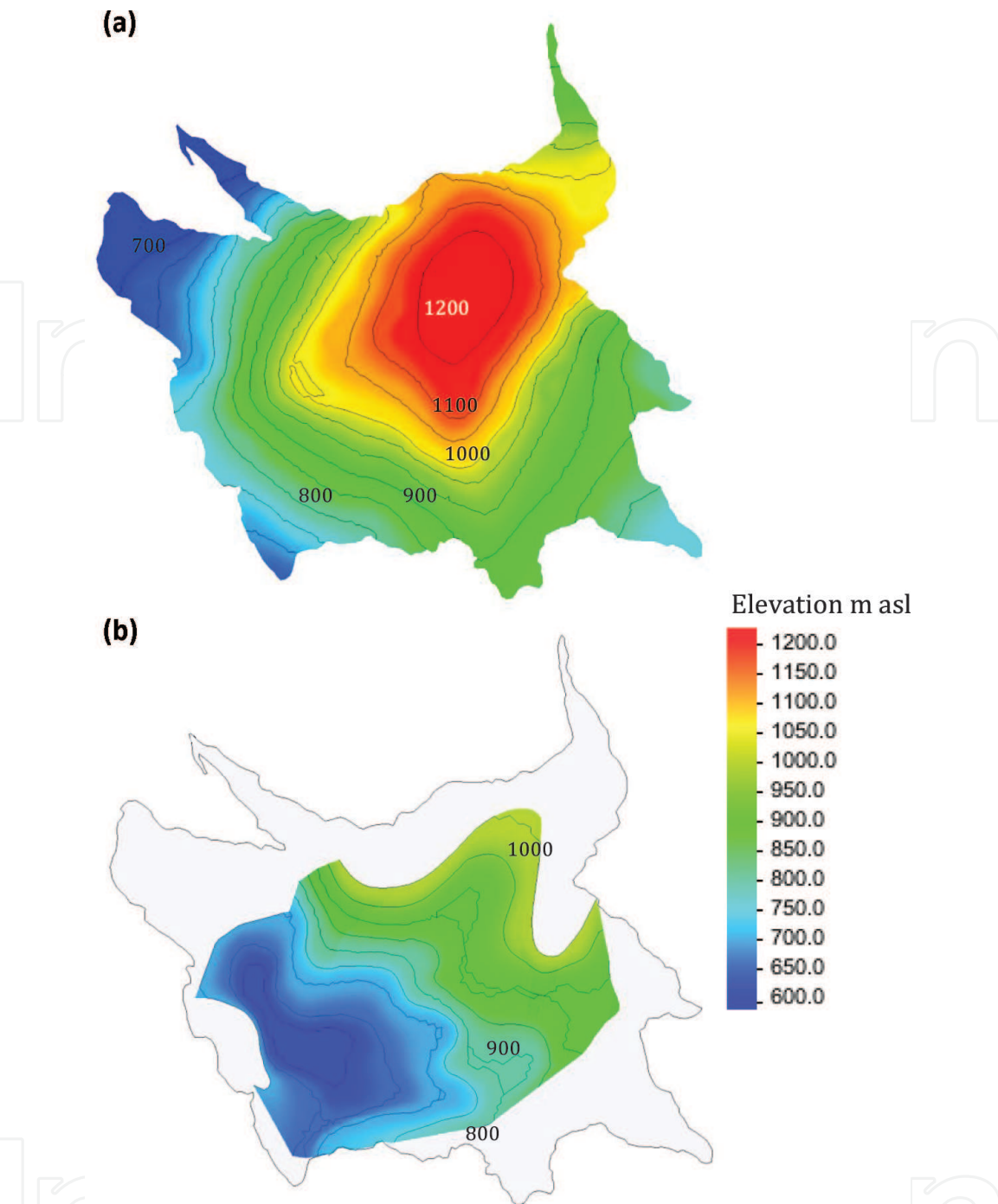
Figure 3. Piezometric surface of the Amiata volcano freshwater aquifer (a) before geothermal exploitation started in 1959 (redrawn from [8]), and (b) after the beginning of geothermal exploitation (redrawn from [24]). The grey-coloured extent of the drawing is the outcrop of volcanic rocks as in (a). The decrease in elevation of the volcanic water table after the beginning of geothermal exploitation is evident and in the range of 100–300 m. Note also in (b) the minimum in the water table that indicates how the water from the superficial aquifer is drained down to the rocks below the volcano, where the hydrothermal system is located.
