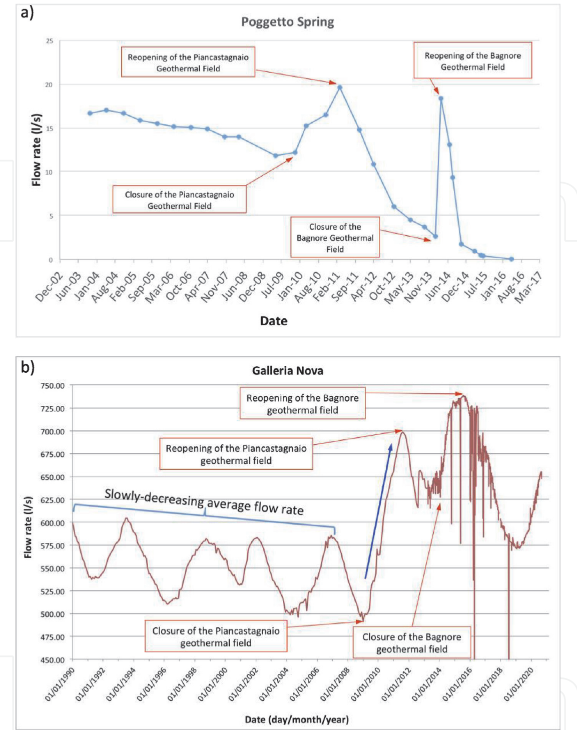
Figure 6. (a) Flowrate versus time of the spring “Poggetto” between 2003 and 2016. The spring flow rate varies inversely with geothermal fluids production of the Mt. Amiata fields. Data courtesy of Ing. Pagano. (b) Flow rate versus time of the galleria Nova drainage tunnel from 1990 to 2020. From 1990 to 2009, the flow rate has clear cycles with a 3–4 year periodicity. The anomalous 30% increase in flow rate that begins in the summer of 2010 (blue arrow) was just before the installation of the first piezometer (Figure 1a) and corresponded to the closure of the Piancastagnaio geothermal field. Also, the closure of the Bagnore geothermal field corresponds to a significant increase in flow rate, while the reopening of the fields matches decreases in flow rate. Data from Regione Toscana—Centro Funzionale Monitoraggio Idrologico-Idraulico.
