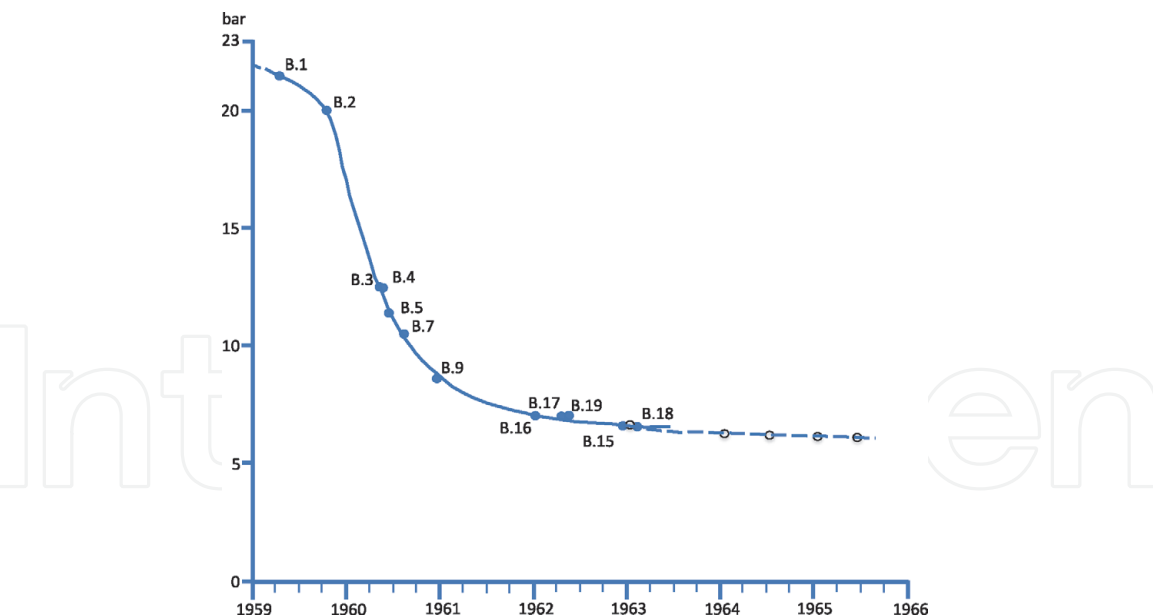
Figure 4. Decrease in the shut-in pressure of the geothermal wells in the reservoirs after the first years of geothermal exploitation (redrawn from [21]). Note that the initial pressure of the wells changes from about 22 bar in 1959 to about 7 bar in 1964. B.# (closed blue dots) are the names of the various wells first drilled at Bagnore. Open dots are non-producing wells.
