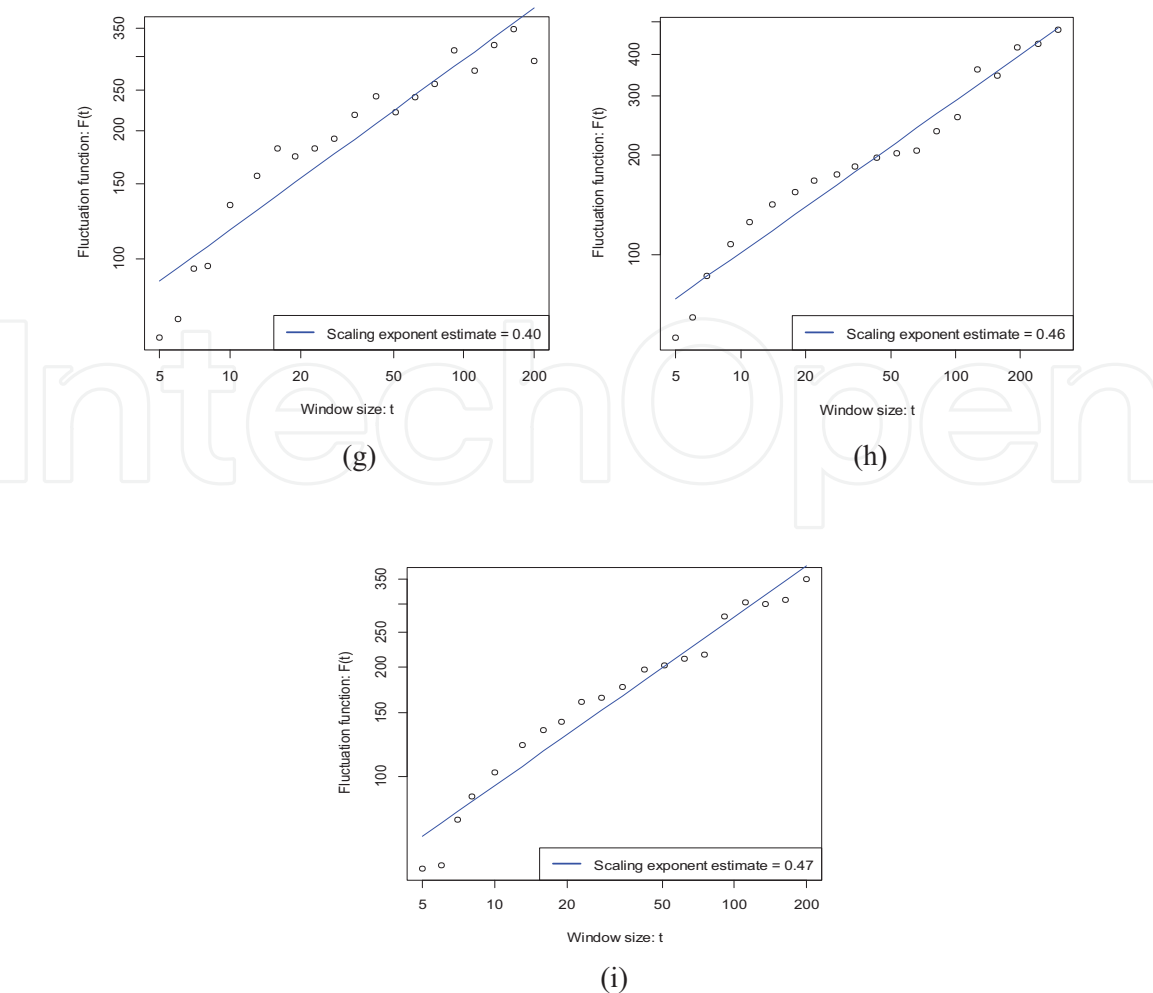
Figure 3. Hurst exponents results based on DFA method for (a) Thiruvallur, (b) Korattur Dam, (c) Ponneri, (d) Poondi (e) Red Hills, (f) Sholingur, (g) Thamarapakkam, (h) Thiruvottiyur, and (i) Vallur Anicut.
