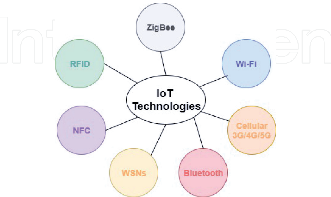
Figure 2. IoT technologies.
