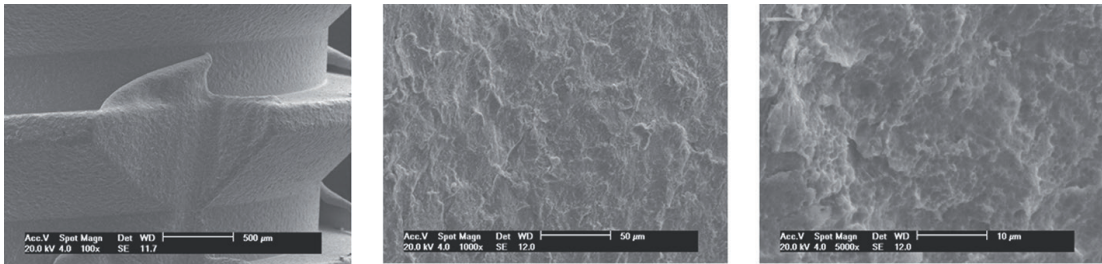
Figure 4. SEM images of a surface treated by sandblasting with aluminum oxide, where we can observe in higher magnifications the presence of sharp edges and other deformations resulting from this surface treatment process.
