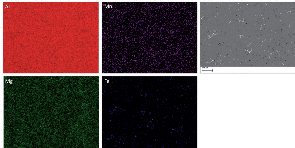
Figure 5. EDS maps analysis of EN AC 51100 bulk.
