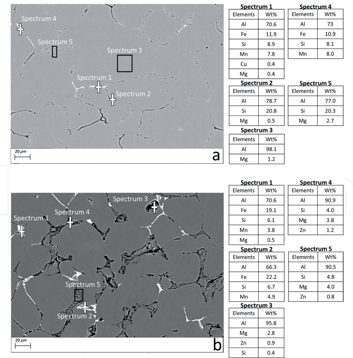
Figure 2. SEM-EDS analysis of specimen EN AC 51100 (a) and EN AC 51100 + Zn (b).
