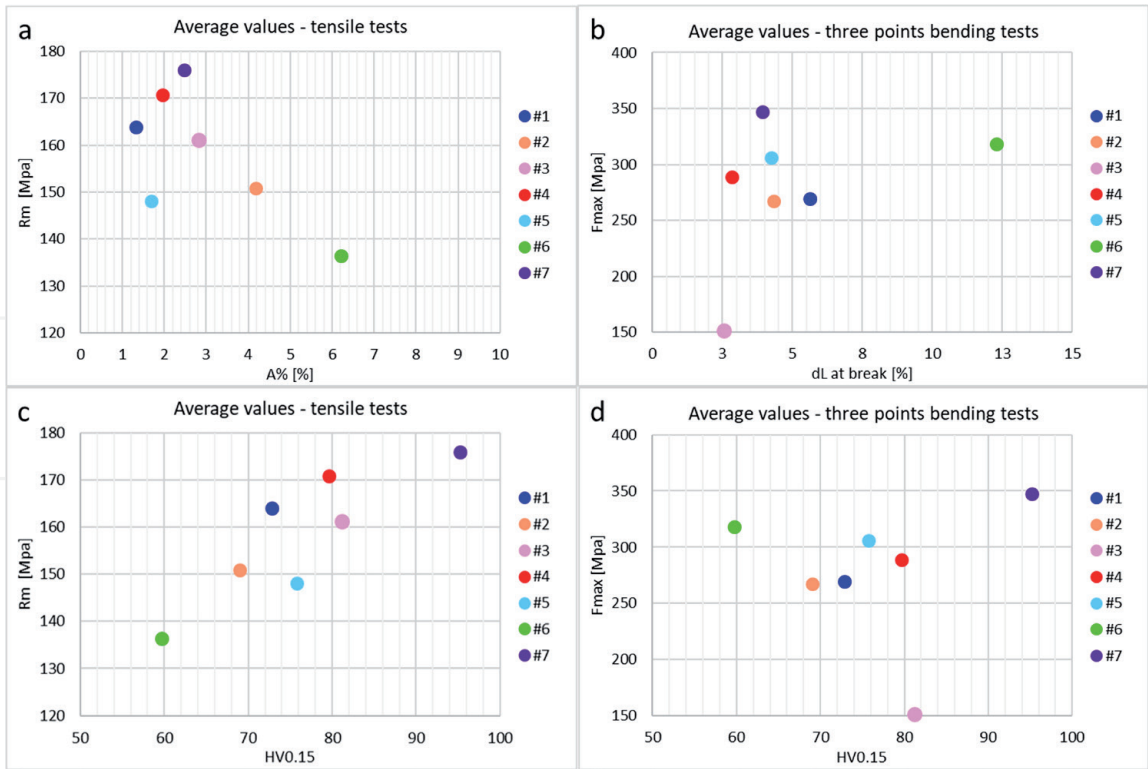
Figure 13. Average values from Tables 3 and 4. a: Average values R_m and A% obtained after tensile tests. b: Average values F_{max} and dL% obtained after bending tests. c: Average values HV0.15 and R_m obtained after tensile tests and microhardness measurements. d: Average values HV0.15 and F_{max} obtained after bending tests and microhardness measurements. FGM, FGM with Zn addition in EN AC 47000 and FGM with Zn addition in both alloys indicated as #1, #2, #3, while EN AC 47000 + Zn, EN AC 51100 + Zn, EN AC 47000, EN AC 51100 indicated as #4, #5, #6, #7.
