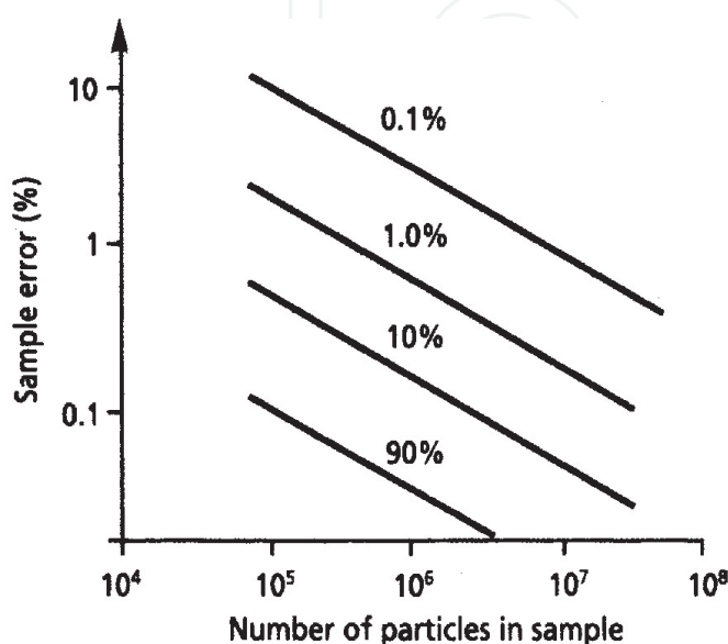
Figure 2. The relationship between sample error, the number of particles in a sample, and different percentages of original material sampled [4].
