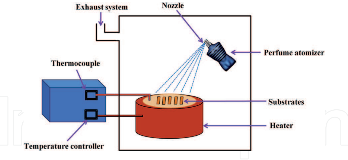
Figure 1. Perfume atomizer spray setup.
