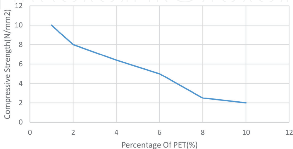
Figure 7. Compressive strength results.
