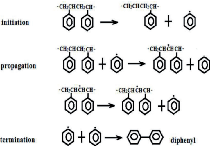
Figure 3. Stages of radical degradation reaction.
