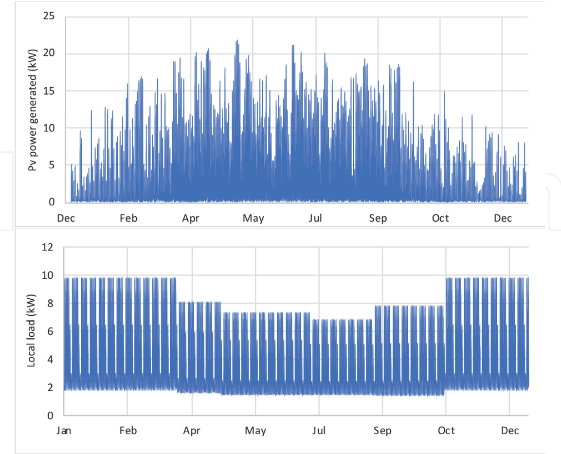
Figure 8. On-site PV generation and local load profiles for all time steps over a year.
