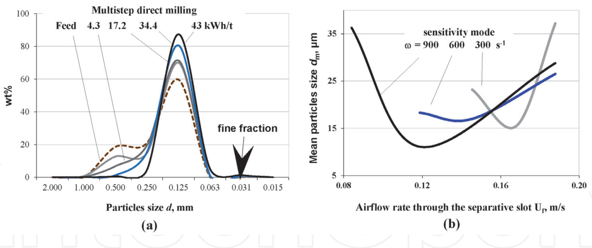
Figure 6. Dependence of the particles size of the IER on the specific energy of treatment E_s and the grinding scheme: (a) Direct multistep milling, (b) results of separative milling with a centrifugal separator (authors image).
