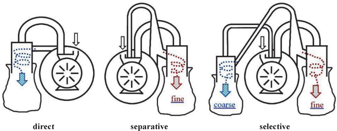
Figure 3. Modes of disintegrator milling (authors image).
