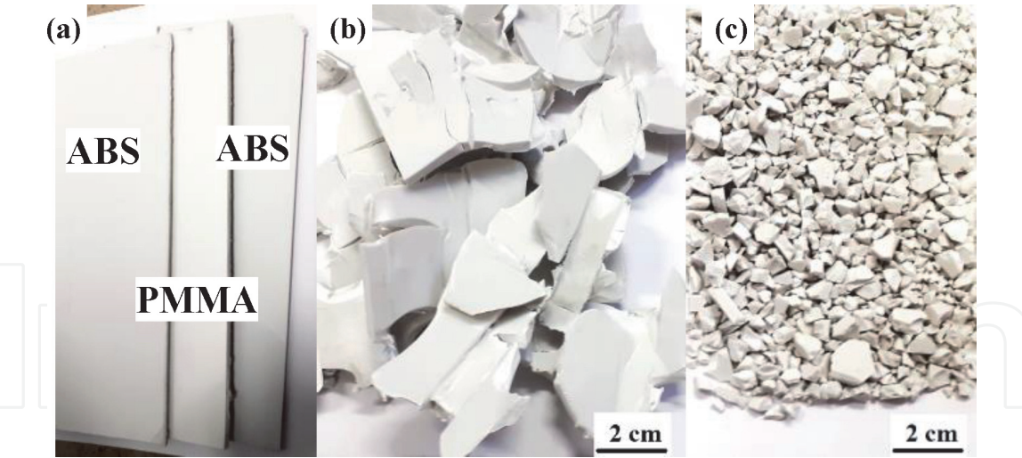
Figure 15. Difference in particle size of the different types of plastics at the same crushing energy E_S = 4.8 \text{ kWh/t} : (a) sheets of material; (b) ductile (ABS); (c) brittle (PMMA) plastics (authors image).
