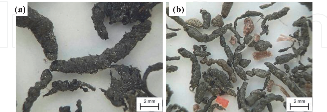
Figure 12. Shear crushing of HDPE by the SD-25 with the gap of the cones: (a) 1 mm; (b) 0.5 mm (authors image).
