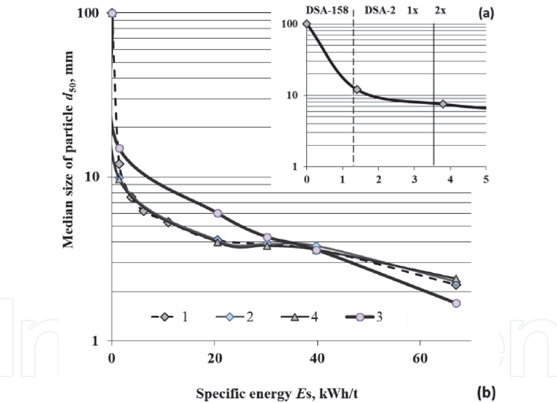
Figure 14. Dependence of the median particle size d_{50} of compound plastic PC + ABS on the specific energy of treatment E_S after precrushing (a) and final multistage milling (b): 1 – PC + ABS monitor housings; 2 – ABS processors; 3 – ABS+HIPS keyboards after precrushing (a) and final multistage milling (b); 4 – PS + ABS+PPE monitor housings [9].
