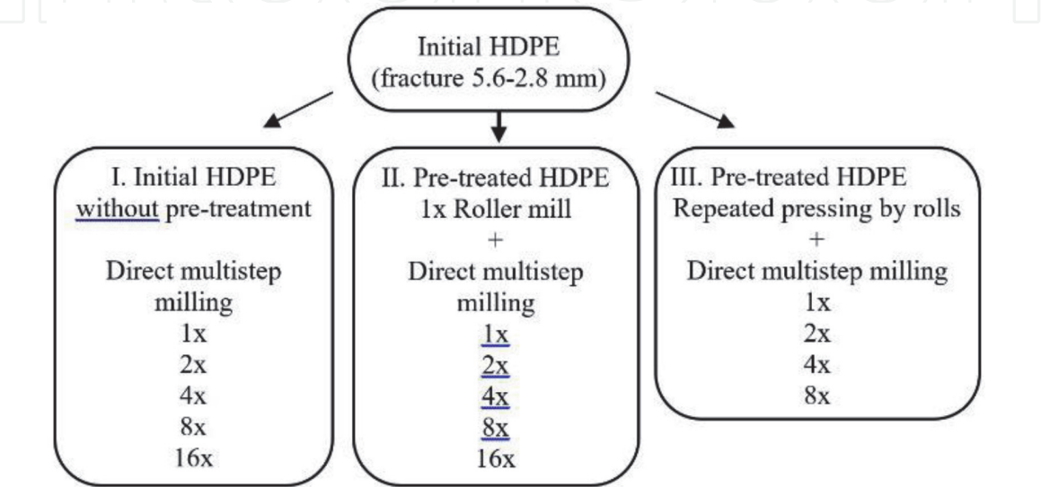
Figure 8. Modes for treatment of HDPE by disintegrator DSL-115: I – Direct multiple grinding; II – Direct multiple grinding of single-deformed material; III – Direct multiple grinding of repeatedly deformed material (authors image).
