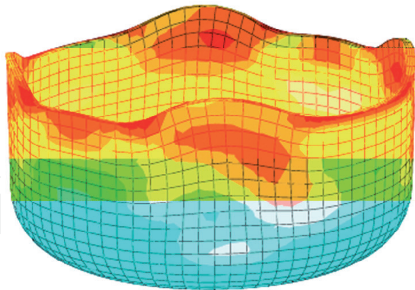
Figure 6. Drawn cup [14].
