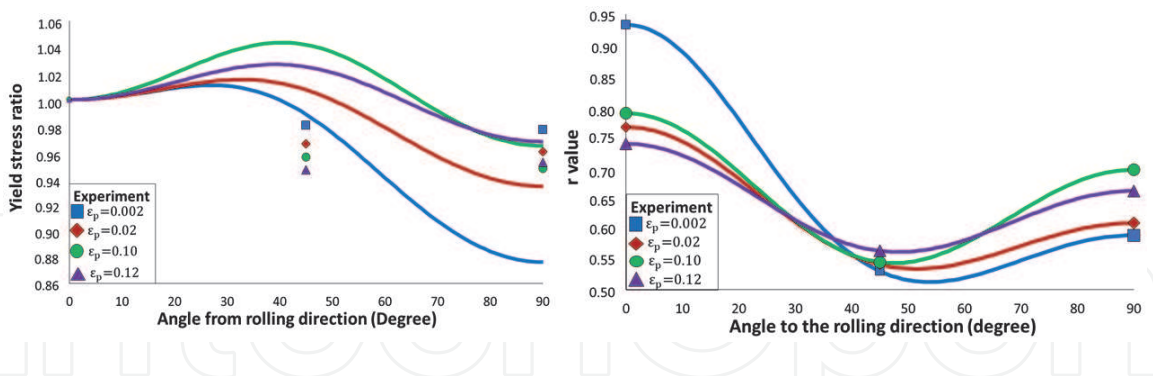
Figure 3. Comparison of the predicted results from P_2 criterion with experiment (a) stress ratio, (b) r -values.
