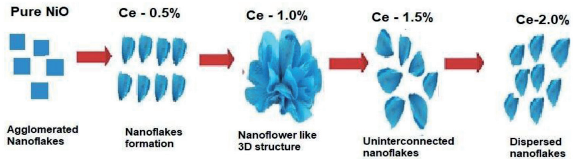
Figure 5. The effect on nanostructure by using various doping percentage in NiO. (Adapted with permission from Ref. [28]. Copyright 2021, Elsevier).
