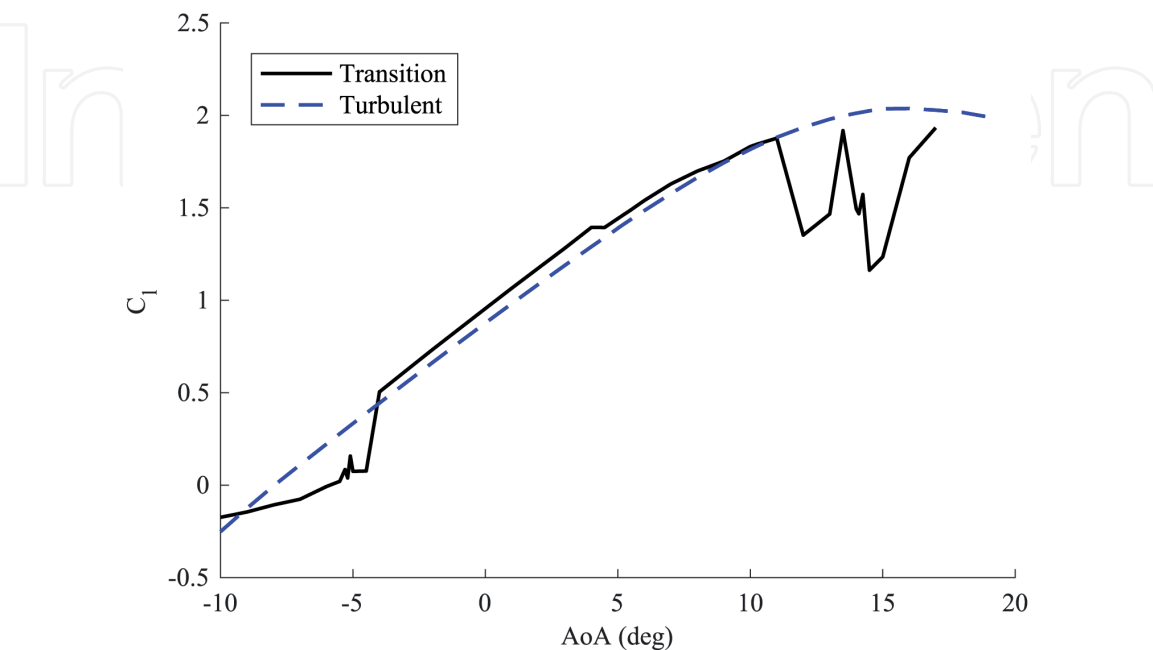
Figure 8. C l comparison between SST and fully turbulent at Re = 2,000,000.
