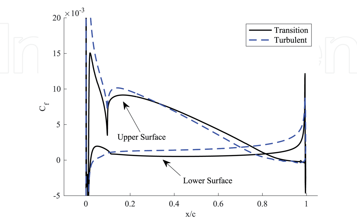
Figure 16. Surface friction coefficients at AoA = 10 degrees, Re = 2,000,000 .
