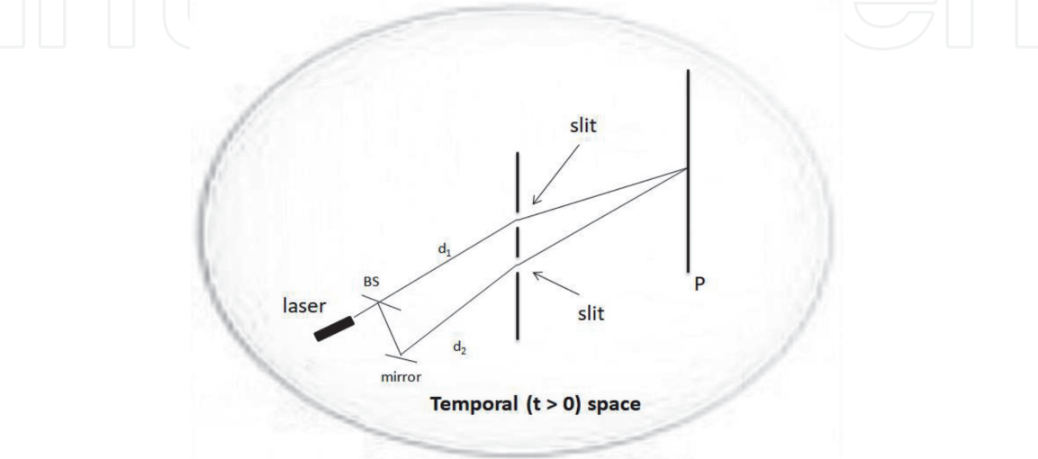
Figure 13. Shows a double-slit experimental setup using a band limited coherent light source.
