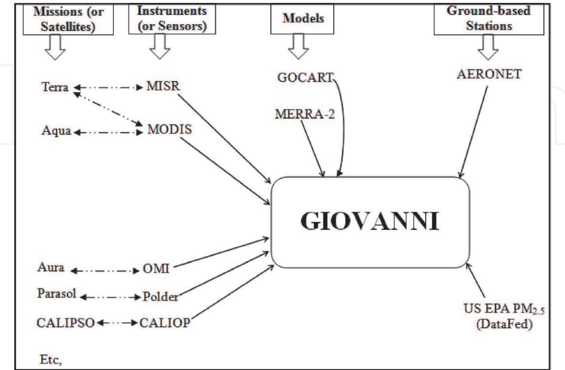
Figure 4. A multi-sensor aerosol data bridge: GIOVANNI.
