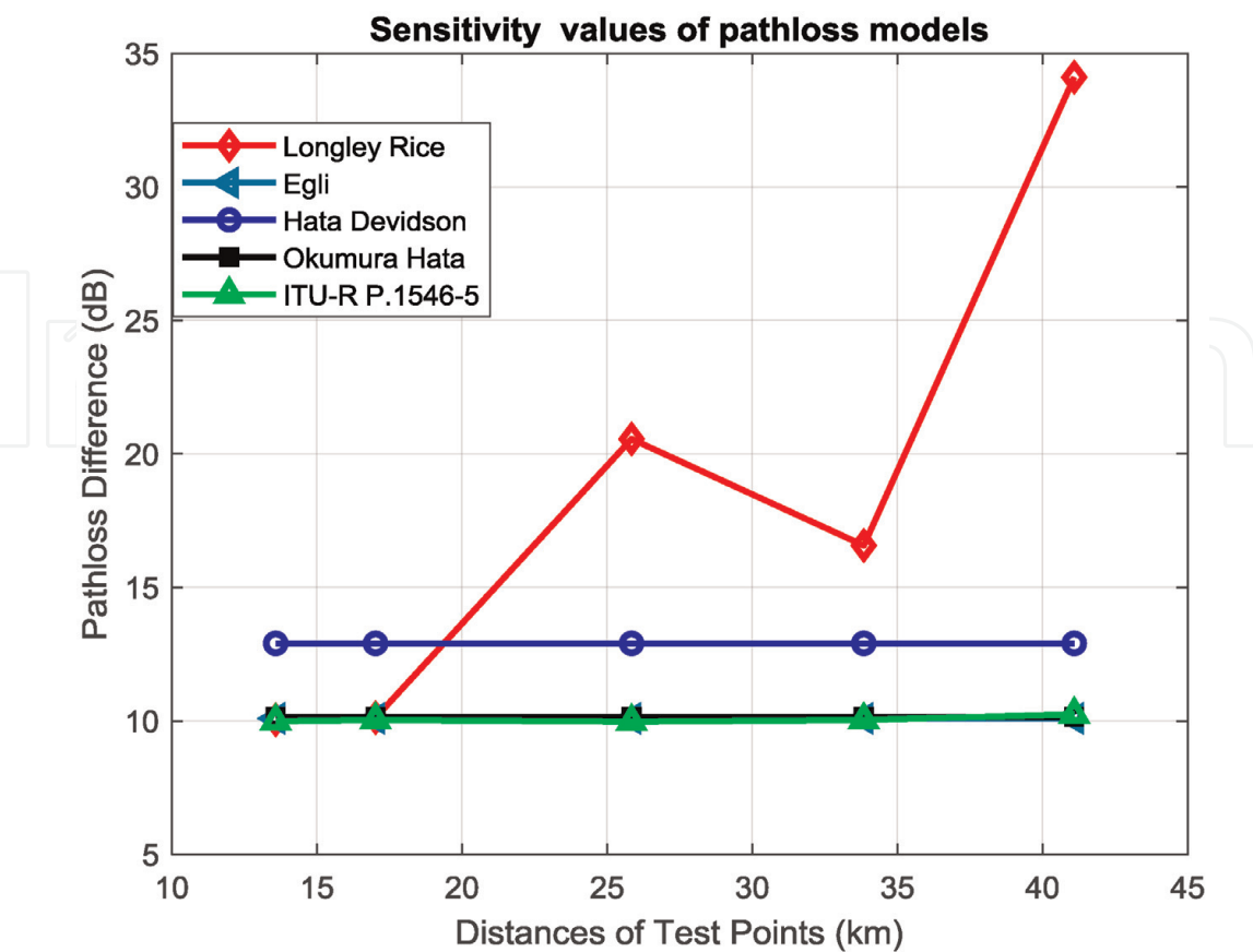
Figure 3. Variations of Pathlosses for VHF and UHF.
