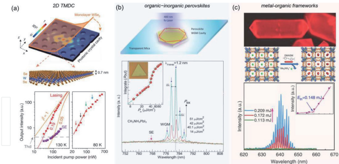
Figure 6. An overview of new materials for nanolasers [50].
