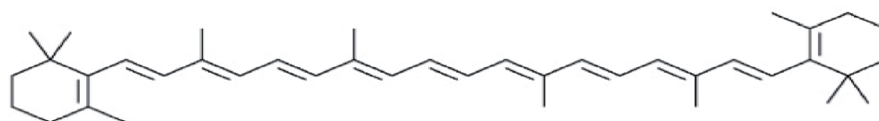
\beta -Carotene
