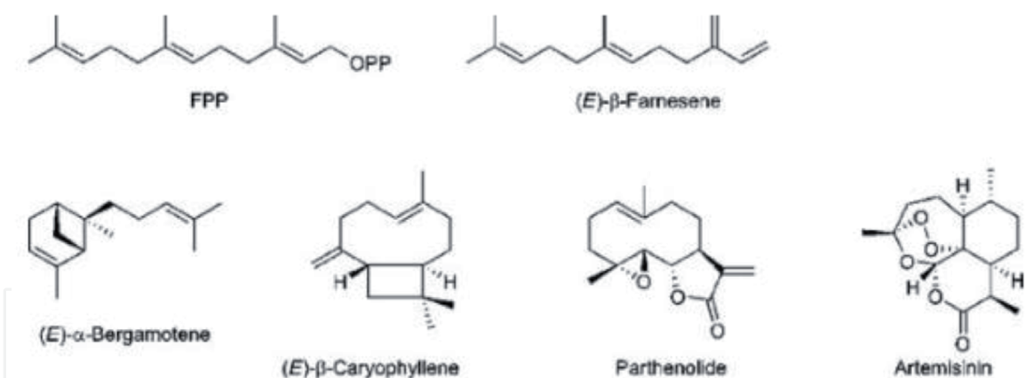
Figure 5. Linear and cyclic sesquiterpenes.
