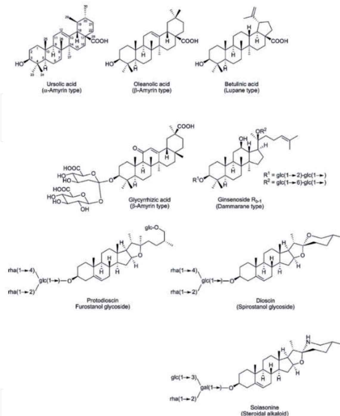
Figure 8. Triterpene and steroid saponins.
