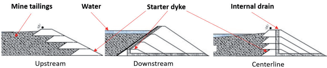
Figure 5. Schematic representation of the construction design of tailings facilities [23].
