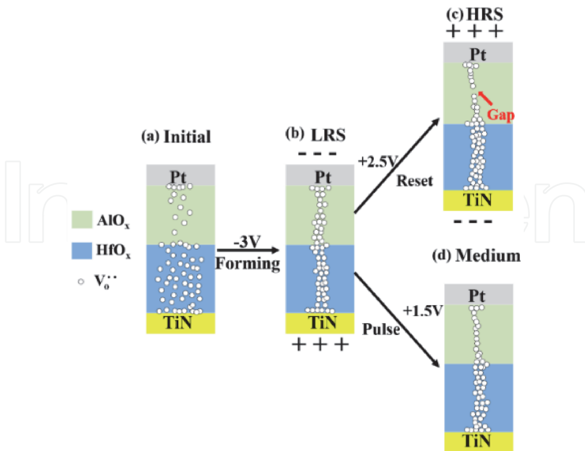
Figure 15. Model of the formation and rupture of a conductive filament consisting of oxygen vacancies. After -3 V forming voltage, the device transfers from an initial resistance state (a) to a low resistance state (LRS) (b); after 2.5 V reset voltage, the device transfers from a low resistance state to a high resistance state (HRS) (c); after 40 continuous pulses ( +1.5 V, 10 ms), the device transfers from LRS to a medium resistance state (d) [17].
