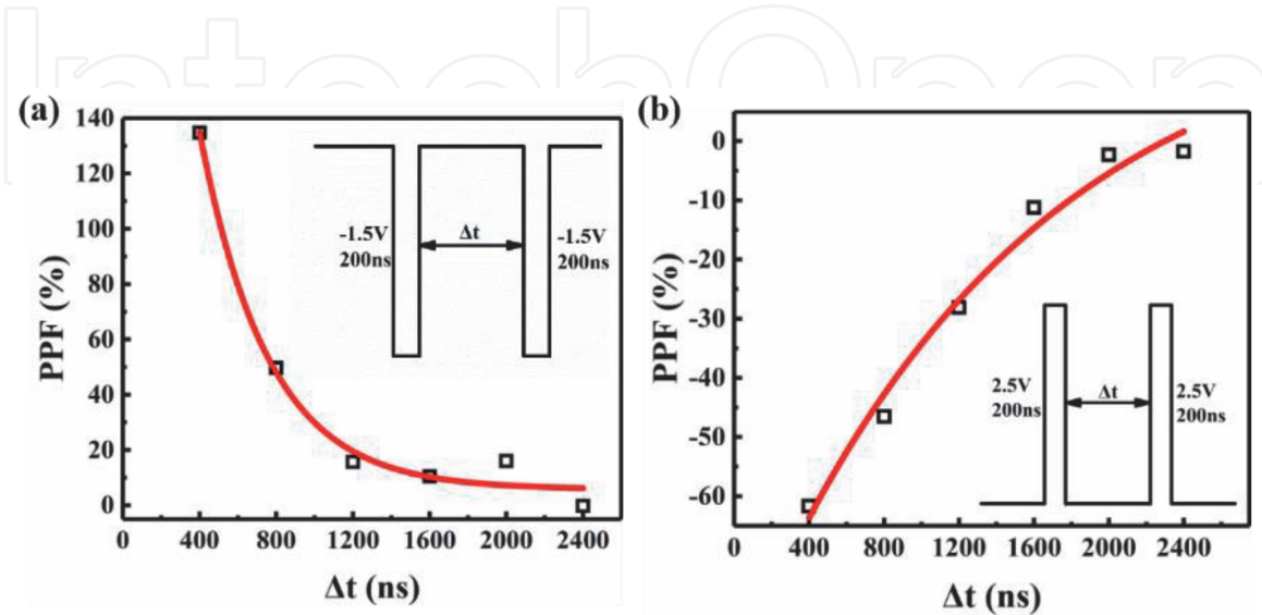
Figure 7. PPF index as the function of the time interval ( \Delta t ) of the \text{Pt}/\text{HfO}_2/\text{HfO}_x/\text{TiN} memristor under negative voltage pulse (a) and positive voltage pulse (b). Black points represent the measurement data, and the red lines represent the fitting data by using Eq. (3). The insets in (a) and (b) record the applied pulse waveforms [20].
