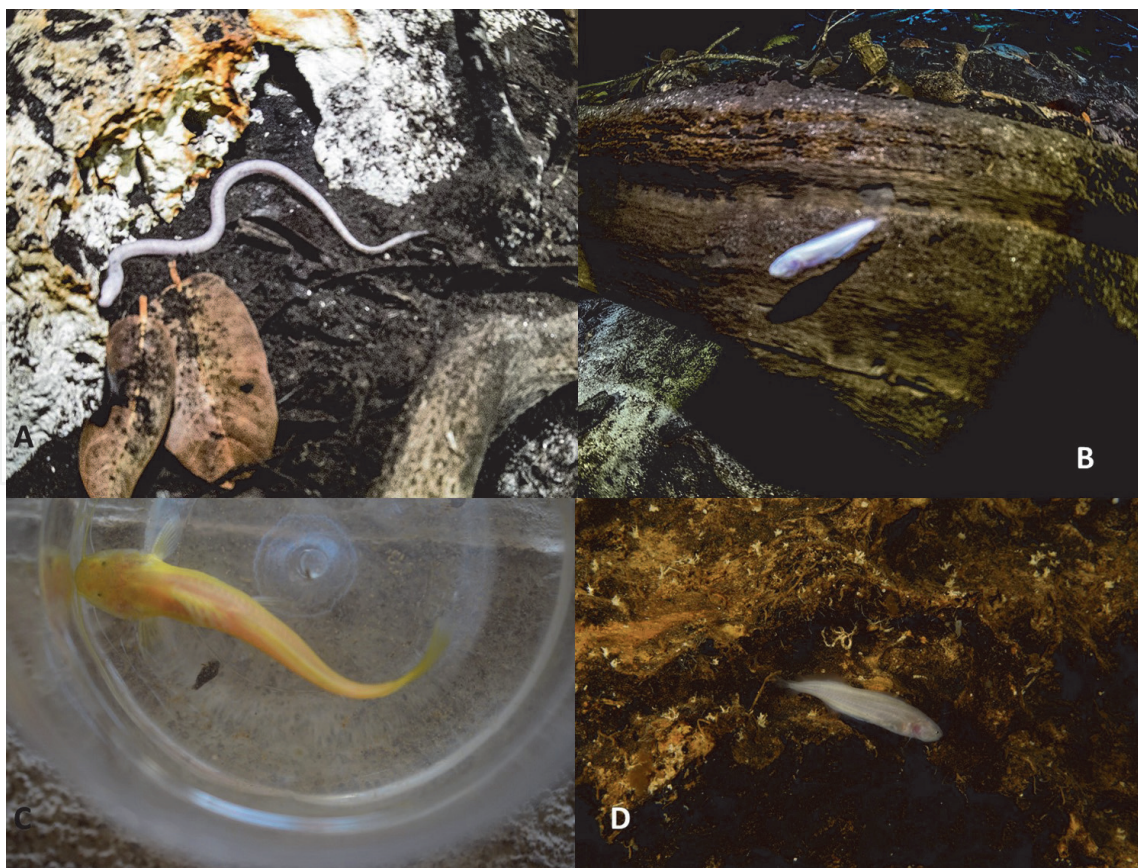
Figure 8. Representative cave fish species in the Mesoamerican region a) Opisthion infernale ; b) Ogilbia pearsei (photo courtesy of Juan Carmona; c) Rhamdia laticauda ; d) fish from Bithynidae family in anchialine ecosystems.
