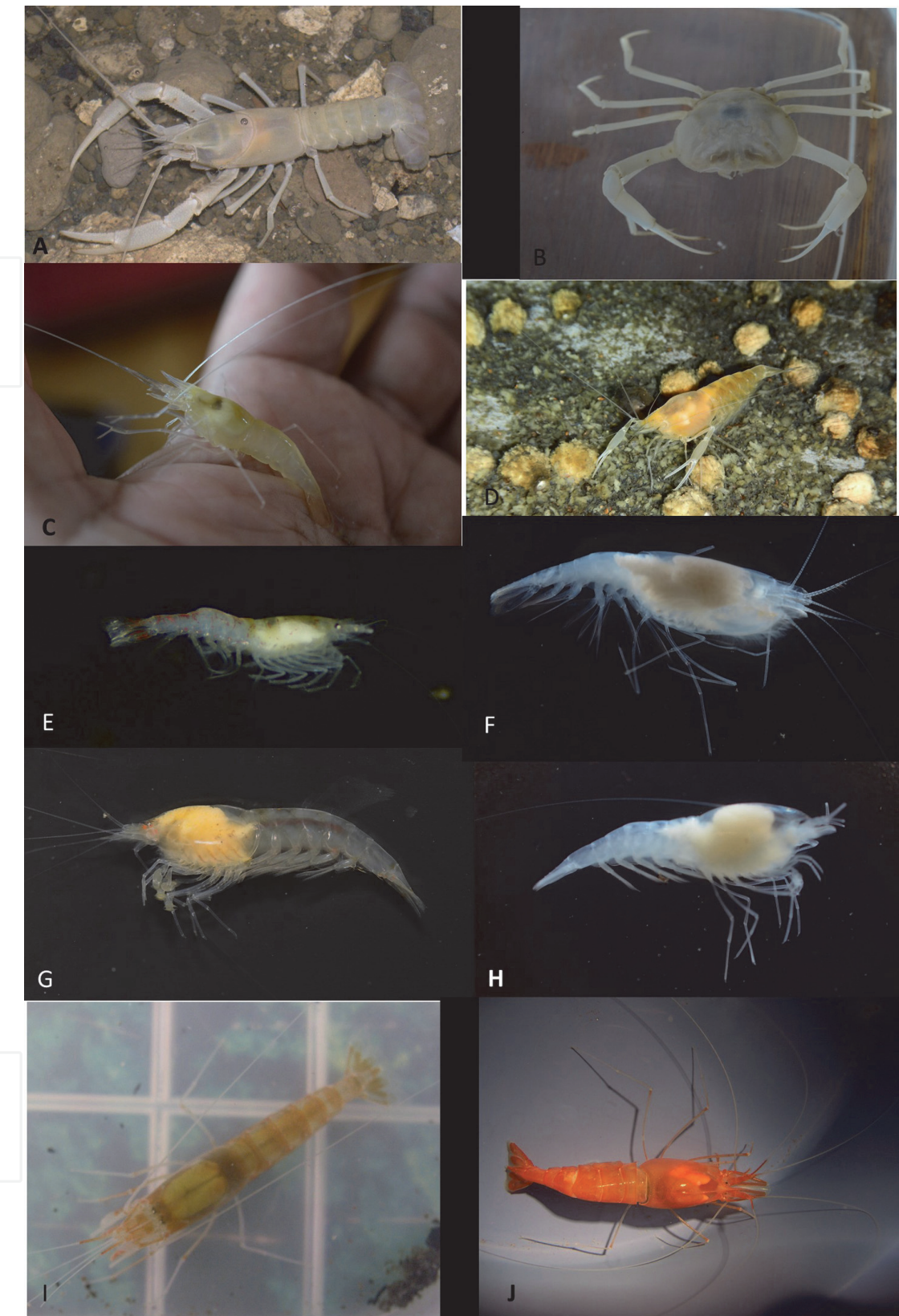
Figure 7. Representative cave crustaceans species in the Mesoamerican region. a) Procambarus sp.; b) Typhlopseudothelphusa acanthochela; c) Macrobrachium catonium; d) Creaseria morleyi (courtesy by Erick Sosa); e) Procaris mexicana; f) Anchialocaris paulini; g) Typhlatya sp.; h) Agostocaris zabaletai; i) Calliasmata nohochi; j) Barbouria cubensis.
