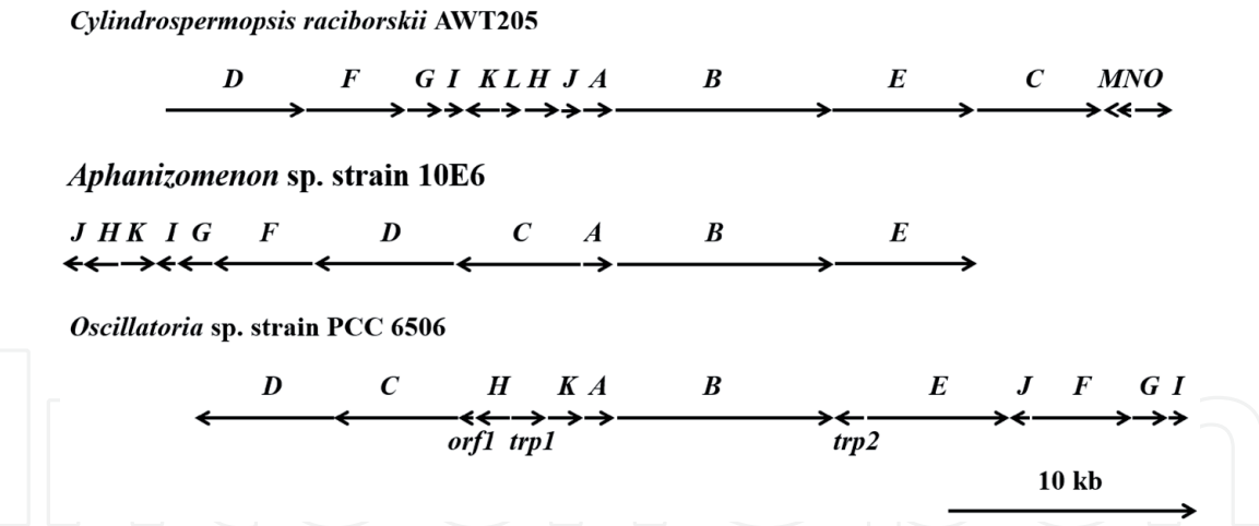
Figure 3. The cylindrospermopsin synthetase gene ( cyr ) clusters of Cylindrospermopsis raciborskii AWT205, Aphanizomenon sp. strain 10E6, and Oscillatoria sp. strain PCC 6506. Each gene is indicated by its designated letter above the arrows, and genes shorter than 500 bp are drawn as an arrowhead only. The diagram only exhibits the size and position of each gene without the distances between two adjacent genes. The measuring scale arrow represents 10 kb.
