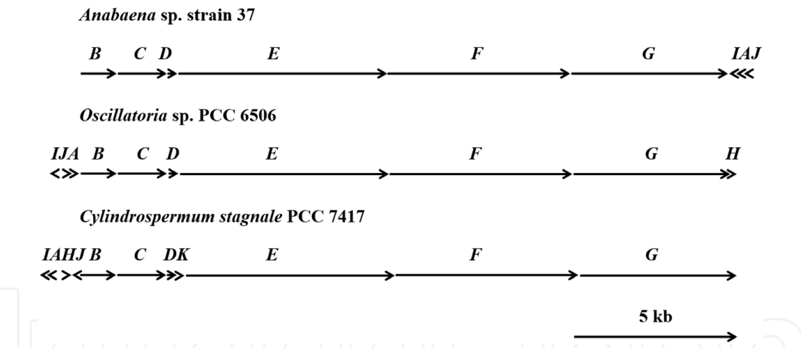
Figure 2. The anatoxin-a synthetase gene ( ana ) clusters of Anabaena sp. strain 37, Oscillatoria sp. PCC 6506, and Cylindrospermum stagnale PCC 7417. Each gene is indicated by its designated letter above the arrows, and genes shorter than 250 bp are drawn as an arrowhead only. The diagram only exhibits the size and position of each gene without the distances between two adjacent genes. The measuring scale arrow represents 5 kb.
