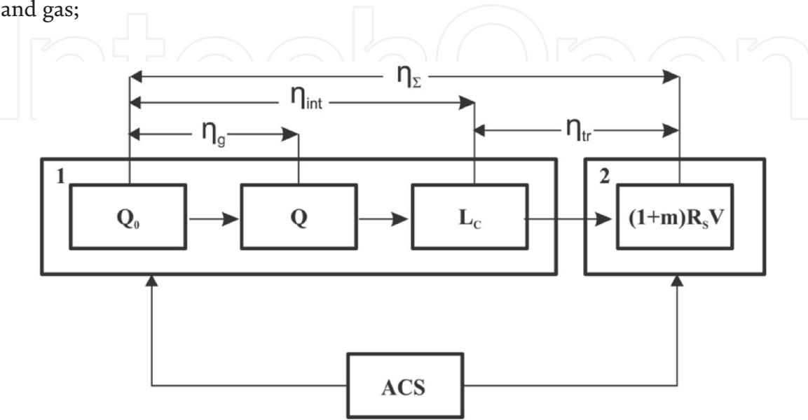
Figure 1. Simplified diagram of the energy balance of a direct reaction GTE: 1- heat engine; 2 - propulsion device; ACS - automatic control system.
