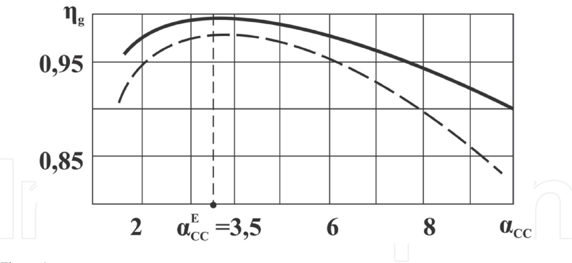
Figure 8. Typical characteristic of the combustion chamber is represented in the following way: The dependence of the fuel combustion efficiency ( \eta_g ) from the excess air ratio in the combustion chamber ( \alpha_{cc} ). The calculated excess air ratio for a given combustion chamber is \alpha_{cc}^E = 3,5 , ————— T_{Cmax}^* , - - - - T_{Cmin}^* .
