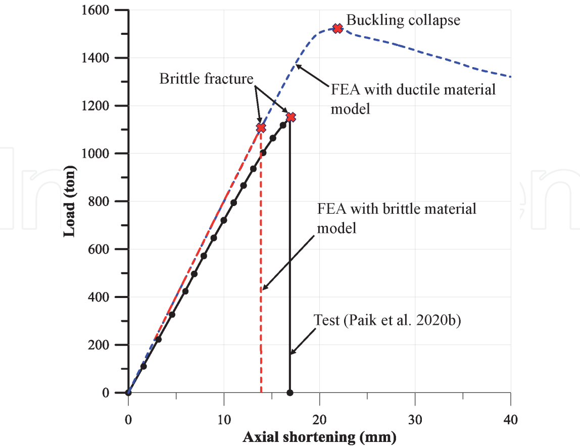
Figure 19. Comparison of the load-axial shortening curves from the test and the FE analysis with the simplified brittle material model.
