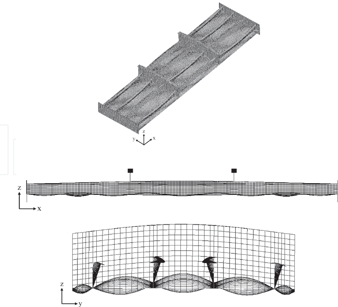
Figure 15. Welding-induced initial deformations applied to the FE model (with an amplification factor of 100 for plating and column-type, and 20 for sideways initial deformations).
