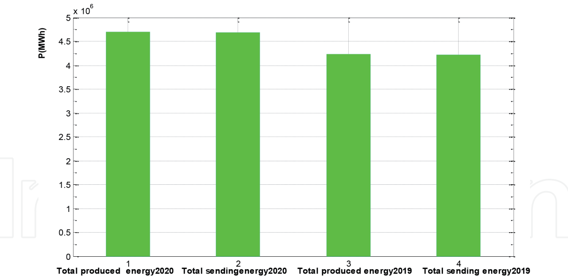
Figure 11. Comparative of Western Mountain power plant production between 2019 & 2020.
