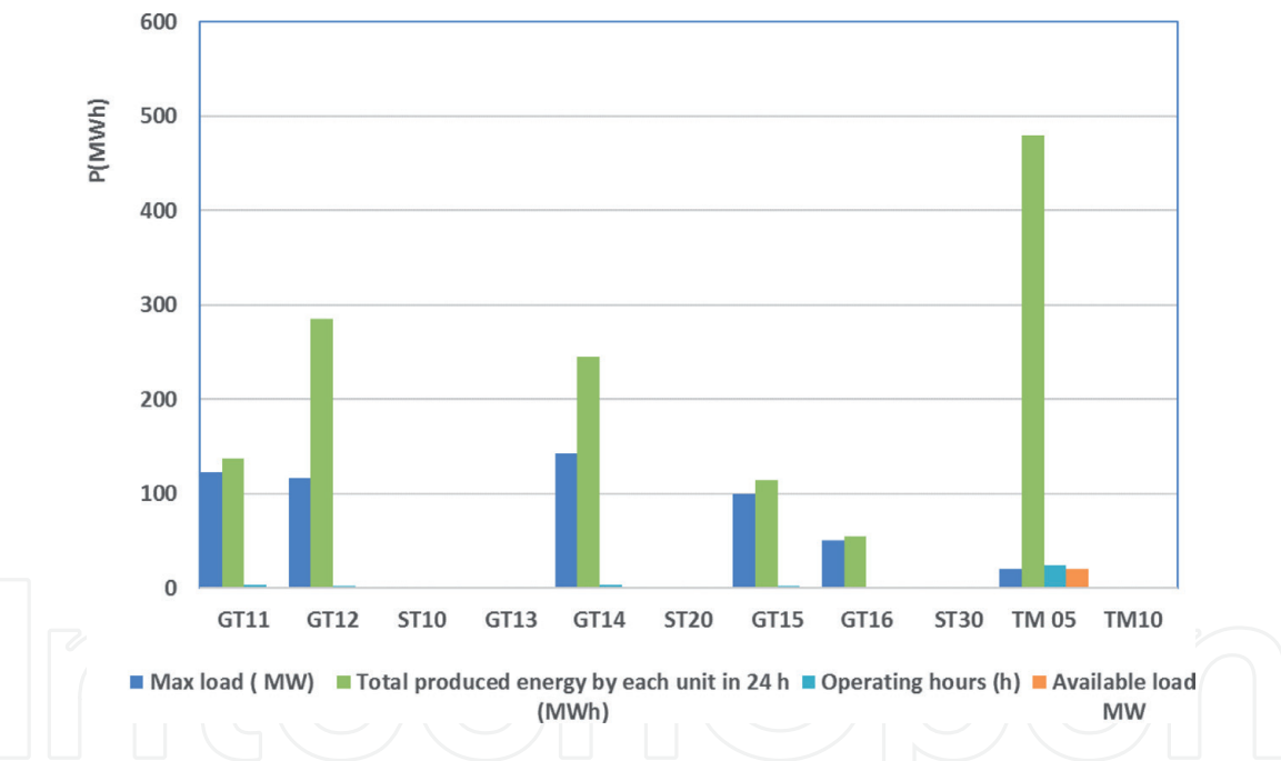
Figure 4. The statu of the nine units on the day of blackout 03-08-2019.
