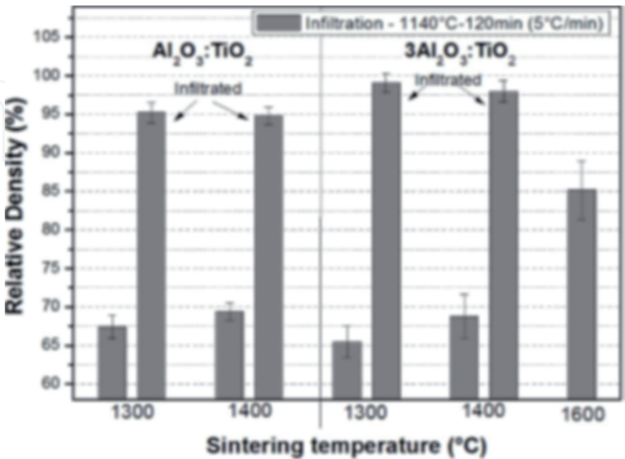
Figure 6. Variation of relative density with sintering temperature of the Al 2 O 3 -TiO 2 and 3Al 2 O 3 -TiO 2 composites after glass infiltration [74].
