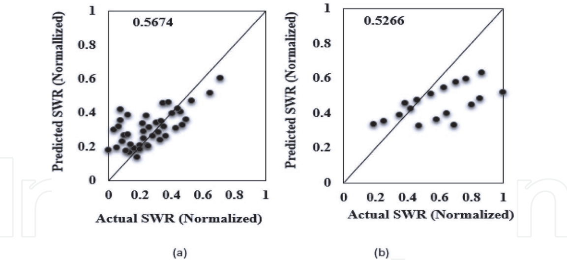
Figure 5. Scatter plot of MLR model in (a) training and (b) testing stages.
