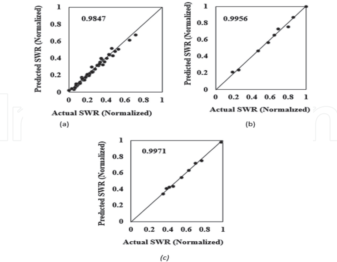
Figure 7. Scatter plot of ANFIS model in (a) training (b) validation and (c) testing.
