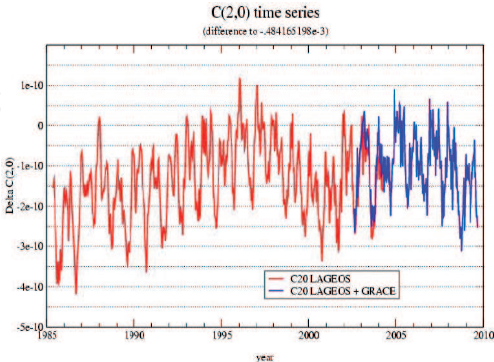
Figure 1. Time variations of the C_{20} coefficient (representing Earth's flatness) determined by analysis of the LAGEOS 1 & 2 satellite telemetry (source: GRGS, Toulouse).
