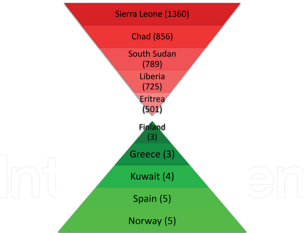
Figure 3. Sand clock of five countries with highest (red) and lowest (green) MMR.
