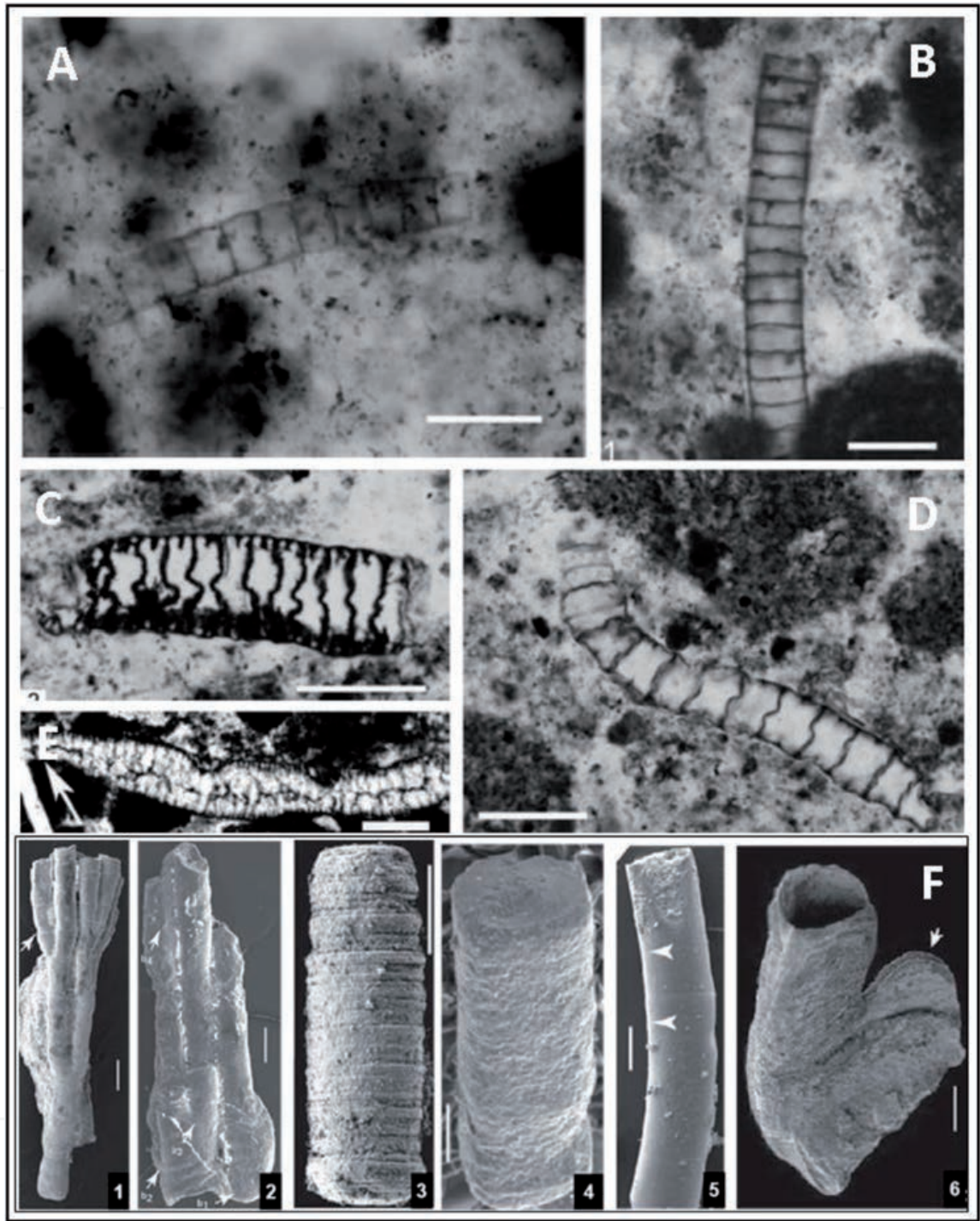
Figure 15. Microphotographs of a set of tubular septate-like bodies thin sections, comparable to Martian samples. Frames A and B: Oscillatoropsis longa Timofeev and Hermann, 1979; scale bars are 50 μm. Frames C-E: Megathrix longus Yin L. from the lower Yurtus and lower Yanjiahe formations; scale bars are 100 μm. Frame F: 1. Ramitubus increscens Liu P., 2008 (scale bar is 200 μm); 2. Ramitubus decrescens Liu P., 2008 (scale bar is 200 μm); 3. Sinocyclocyclicus guizhouensis Xue Y., 1992 (scale bar is 100 μm); 4. Quadratitubus orbignatus Xue Y., 1992 (scale bar is 100 μm); 5. Crassitubus costatus Liu P., 2008 (scale bar is 100 μm); 6. Yangtztubus semiteres Liu P., 2008 (This one is silicified and also from Ediacaran Doishantuo Formation; scale bar is 50 μm).
