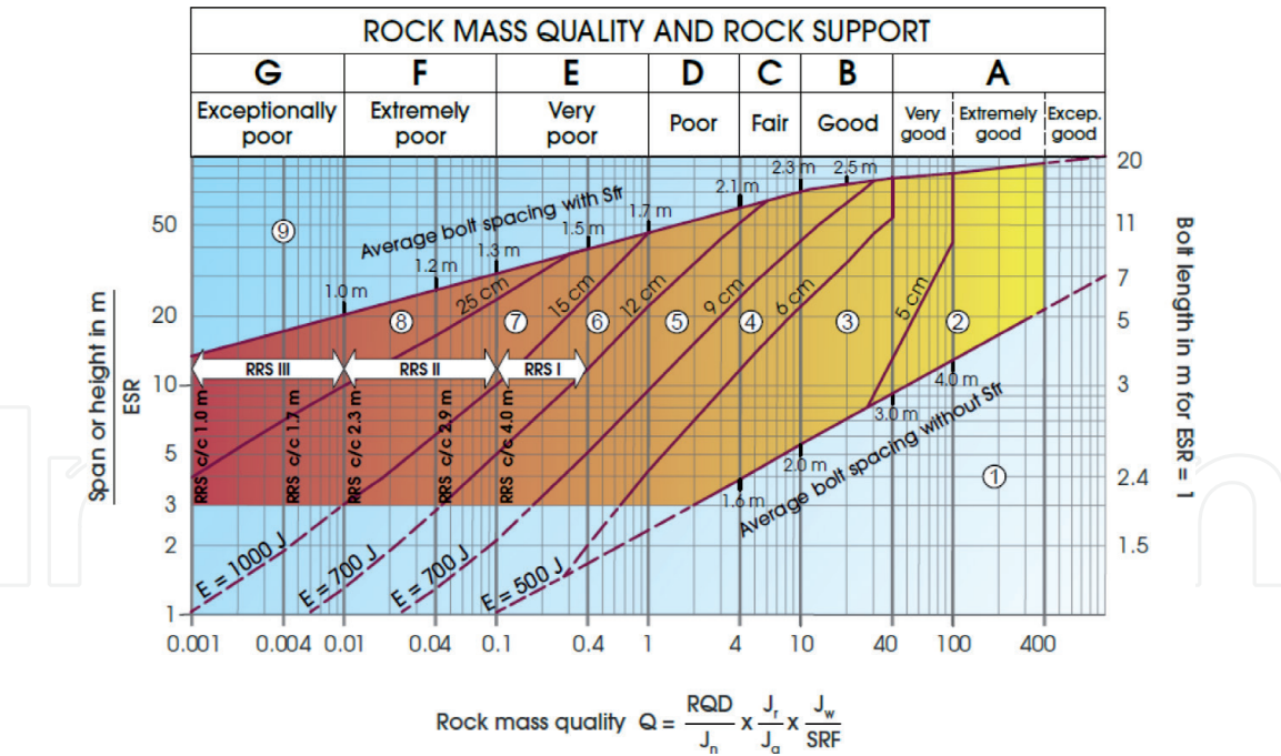
Figure 2. Tunnel support chart based on Q-system [2].
