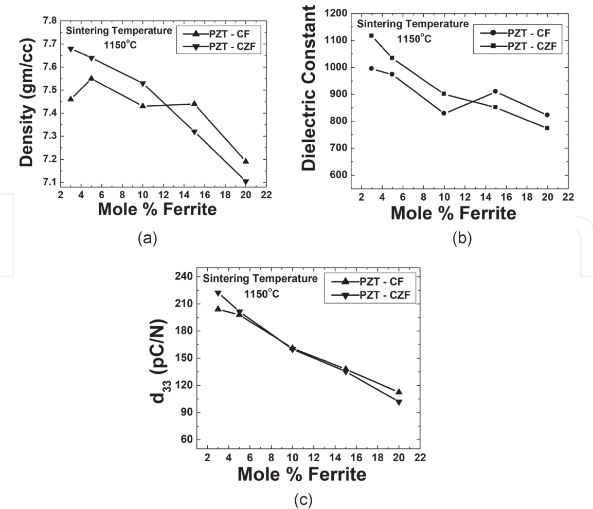
Figure 5. (a), (b) and (c) The density, dielectric constant and piezoelectric constant as a function of mole percent ferrite.
