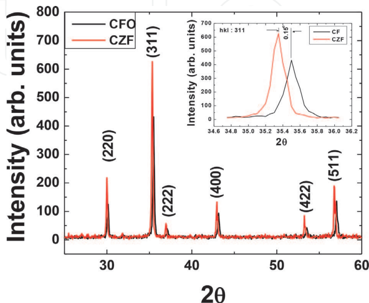
Figure 7. XRD patterns for CFO and CZF particles.
