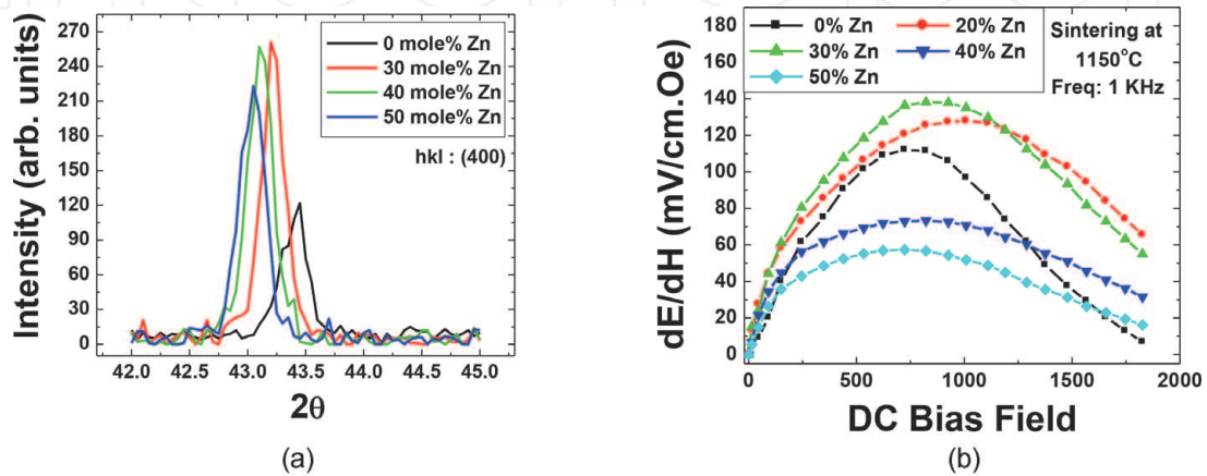
Figure 4. Effect of Zn concentration on (a) peak shift of 400 peaks and (b) magnetoelectric coefficient of PZT-20 NZF [25].
