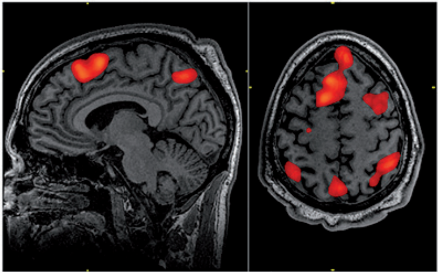
Figure 6. SPM in which the color of pixels is representative of its p -value and, thus, the statistical significance of its activation or deactivation when two or more tasks are compared. From G.Konstantina, CC BY-SA 4.0, via Wikimedia commons.
