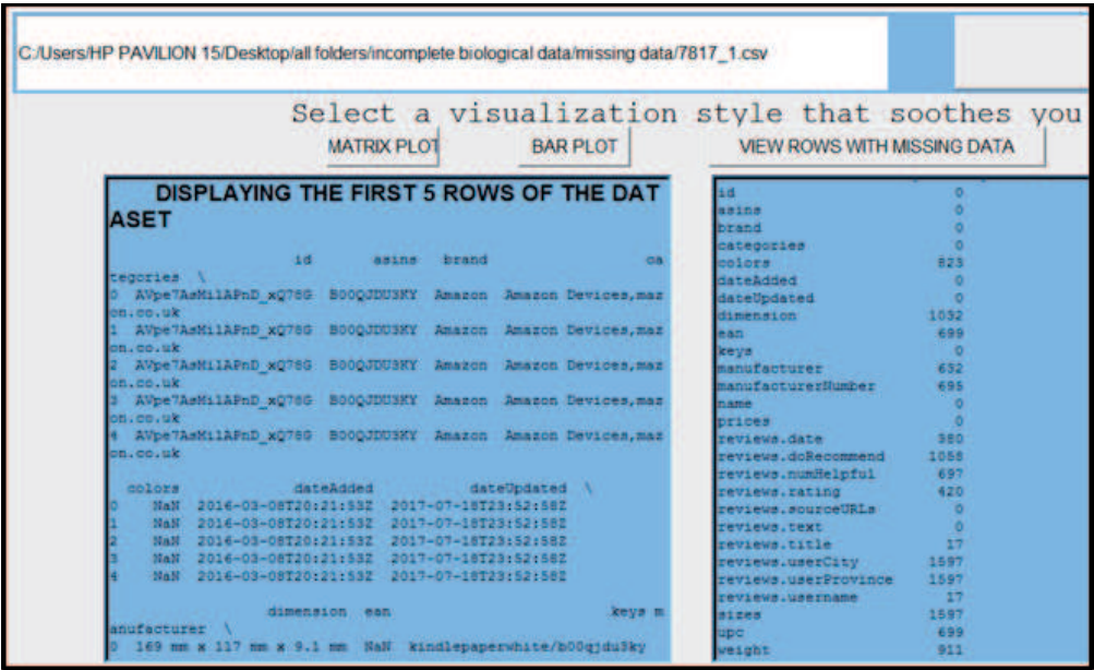
Figure 2. Daxx evaluation pane depicting the number of missing data per investigated column.
