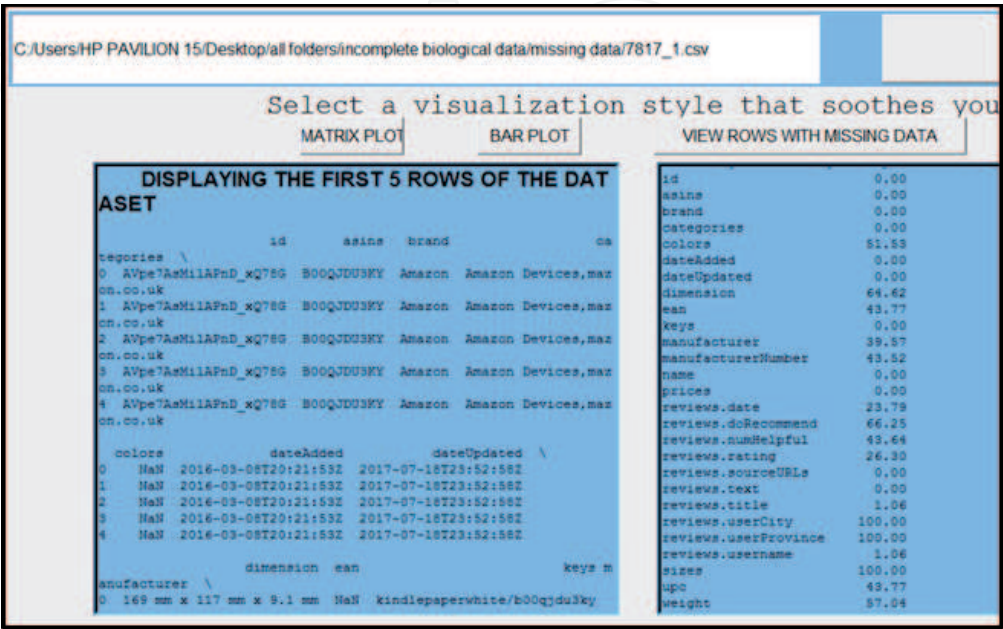
Figure 3. Daxx evaluation pane depicting the percentage of Missingness per investigated column.
