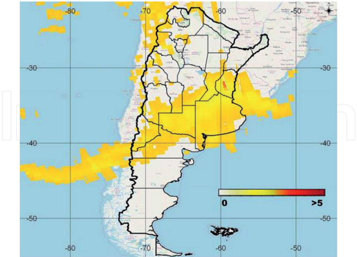
Figure 12. Aerosol Index (AI), calculated by the OMPS sensor measurements for 14 November 2019.
