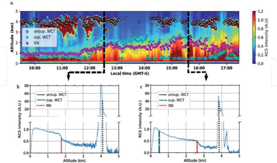
Figure 5. Lidar retrievals for 14 August 2019 [30]. (a) Temporal evolution of the ABL, and (b), (c) Two selected single profiles. They point out different scenarios treated with our method: the measurements exhibit b Profile 1 (12:30 h), a well-mixed layer where NN and sup. WCT values are very similar; and c, Profile 2 (15:40 h), shows conditions where the NN estimation differs from supervised and unsupervised WCT values; the latter profile exhibits an extended ABL a height of about 2.6 km for the NN prediction. The intensity of the signals is given in arbitrary units (a. u.) [31].
